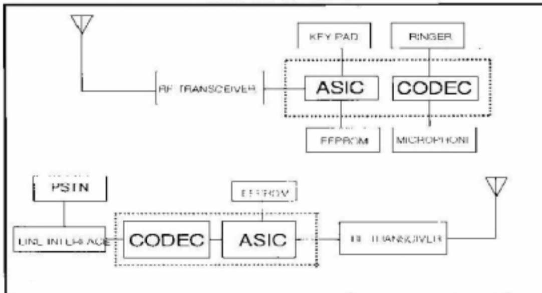
MH9026 System Architecture
