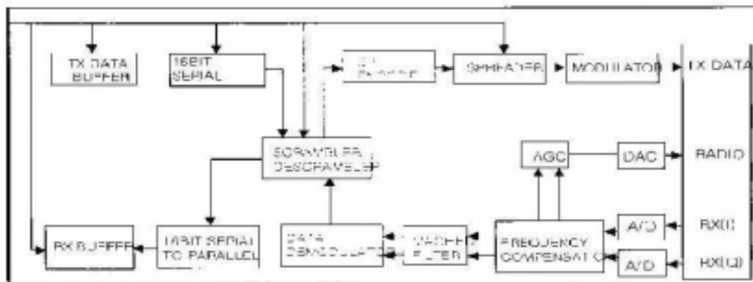
DCT Spread Spectrum Engine Block Diagram
