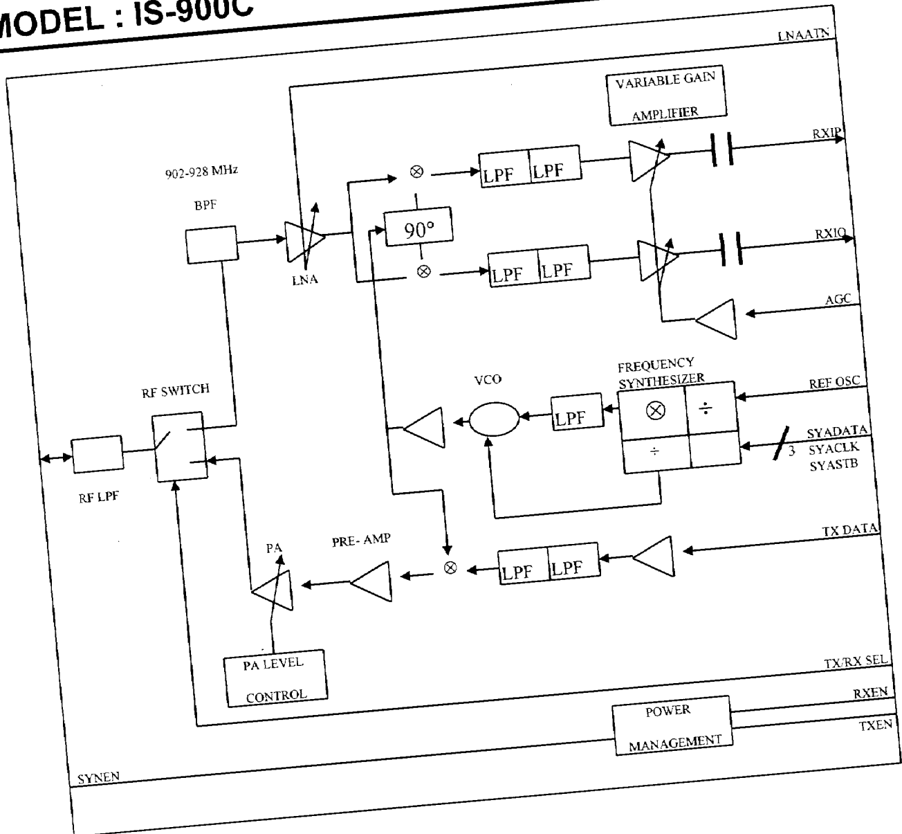
RF Block Diagram
