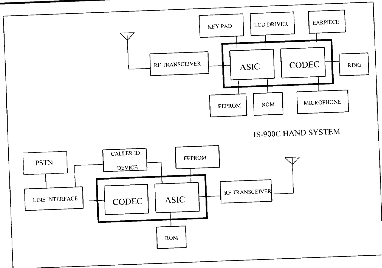
IS-900C System Architecture
