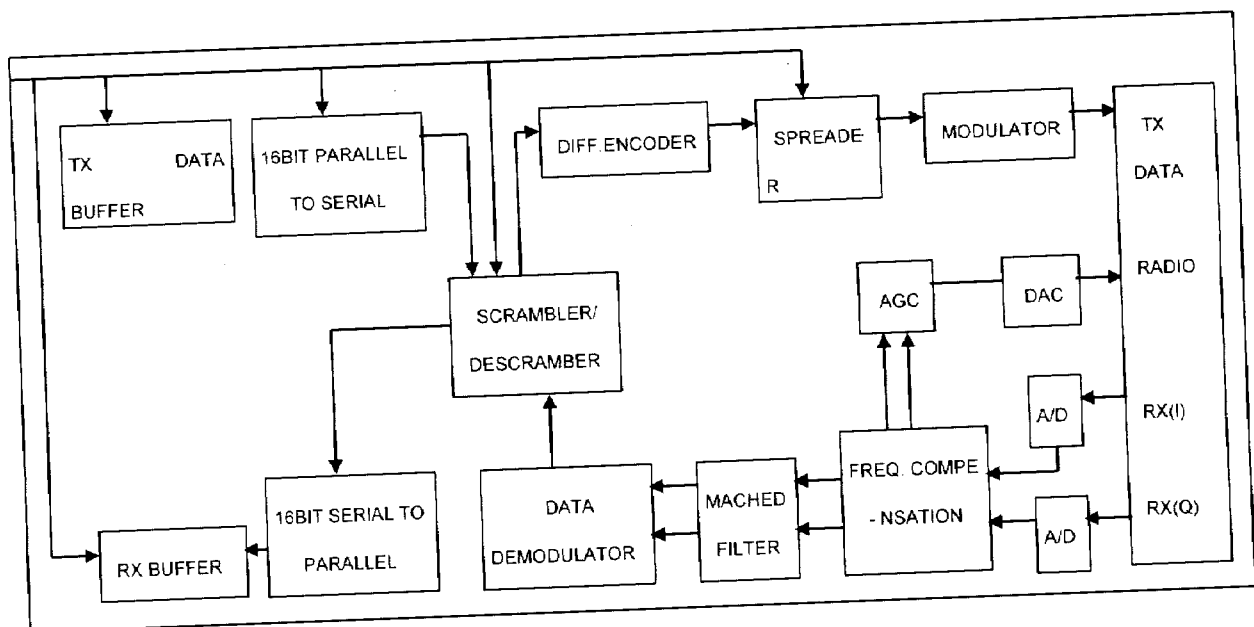
DCT Spread Spectrum Engine Block Diagram
