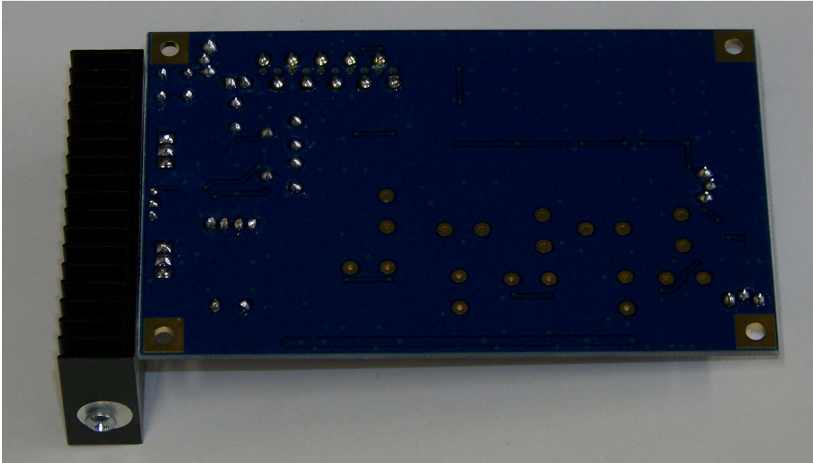
10 WATT PA LOWPASS FILTER BOARD BOTTOM
