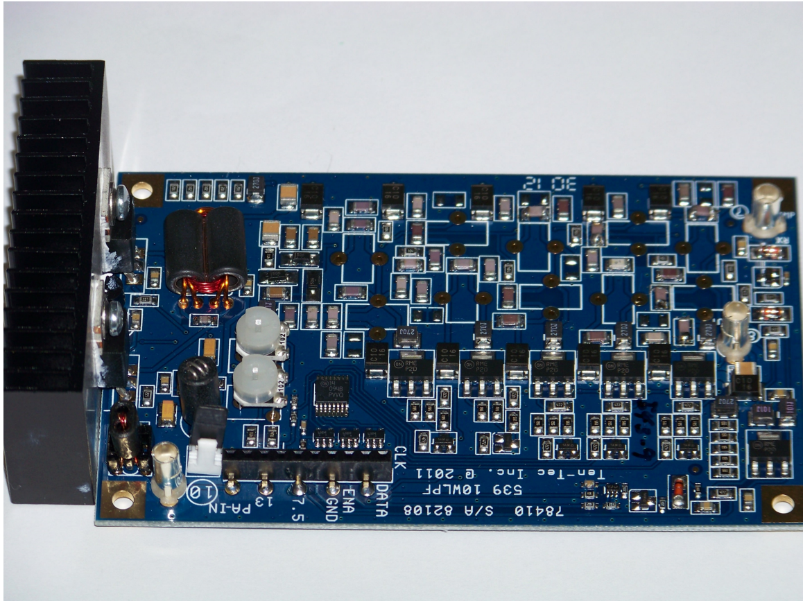
10 WATT PA LOWPASS FILTER BOARD TOP
