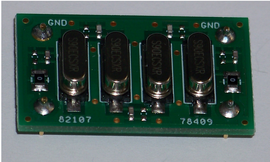
700 Hz FILTER BOARD TOP
