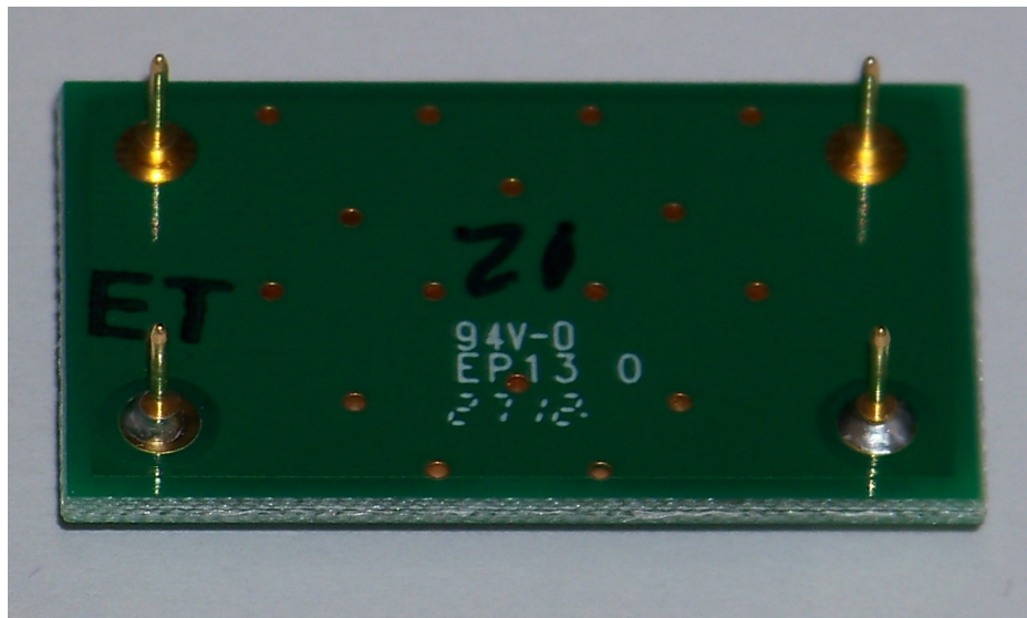
2800 Hz FILTER BOARD BOTTOM
