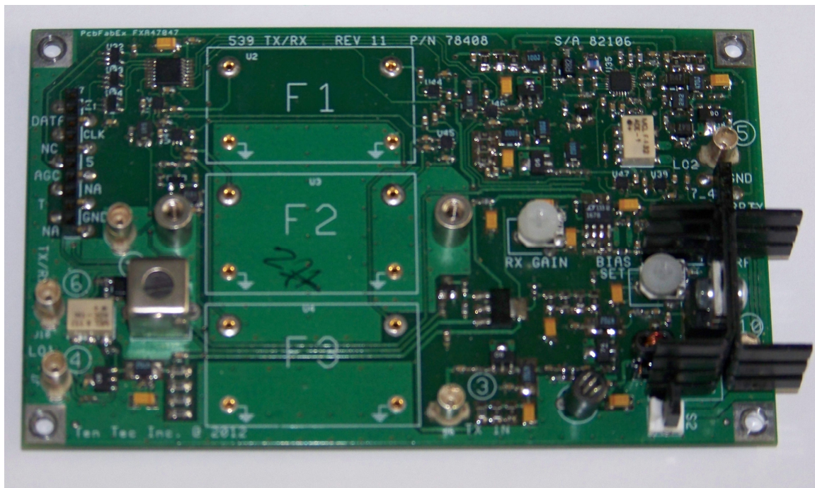
TX/RX BOARD WITHOUT FILTERS TOP
