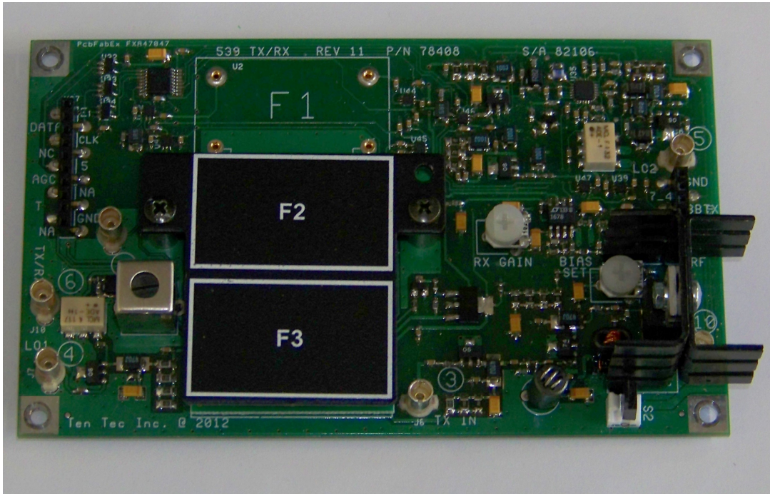
TX/RX BOARD WITH FILTER COVER TOP
