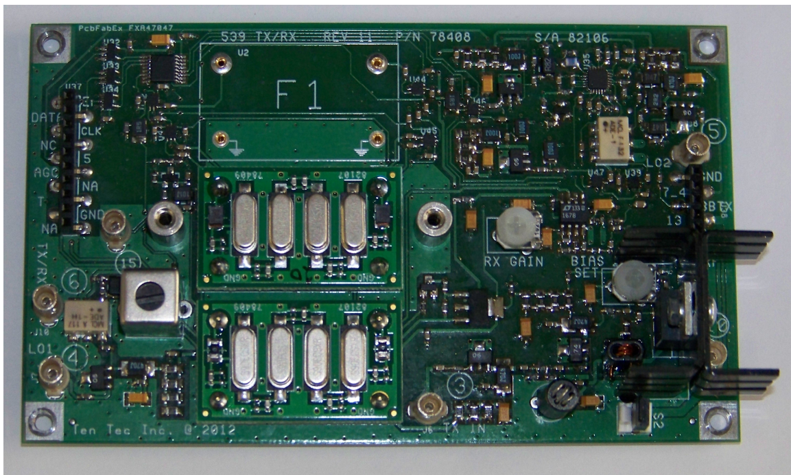
TX/RX BOARD WITHOUT FILTER COVER BOTTOM
