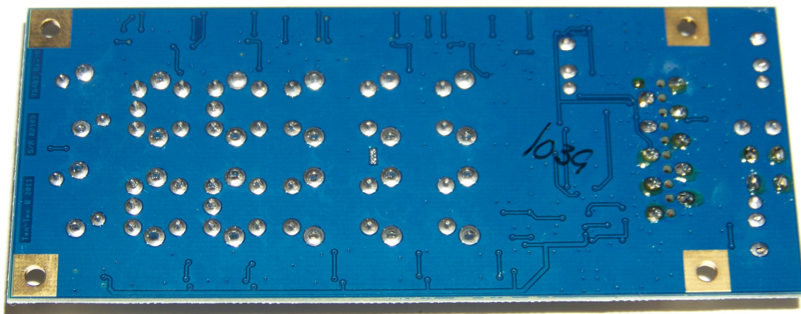
PRESELECTOR BOARD BOTTOM
