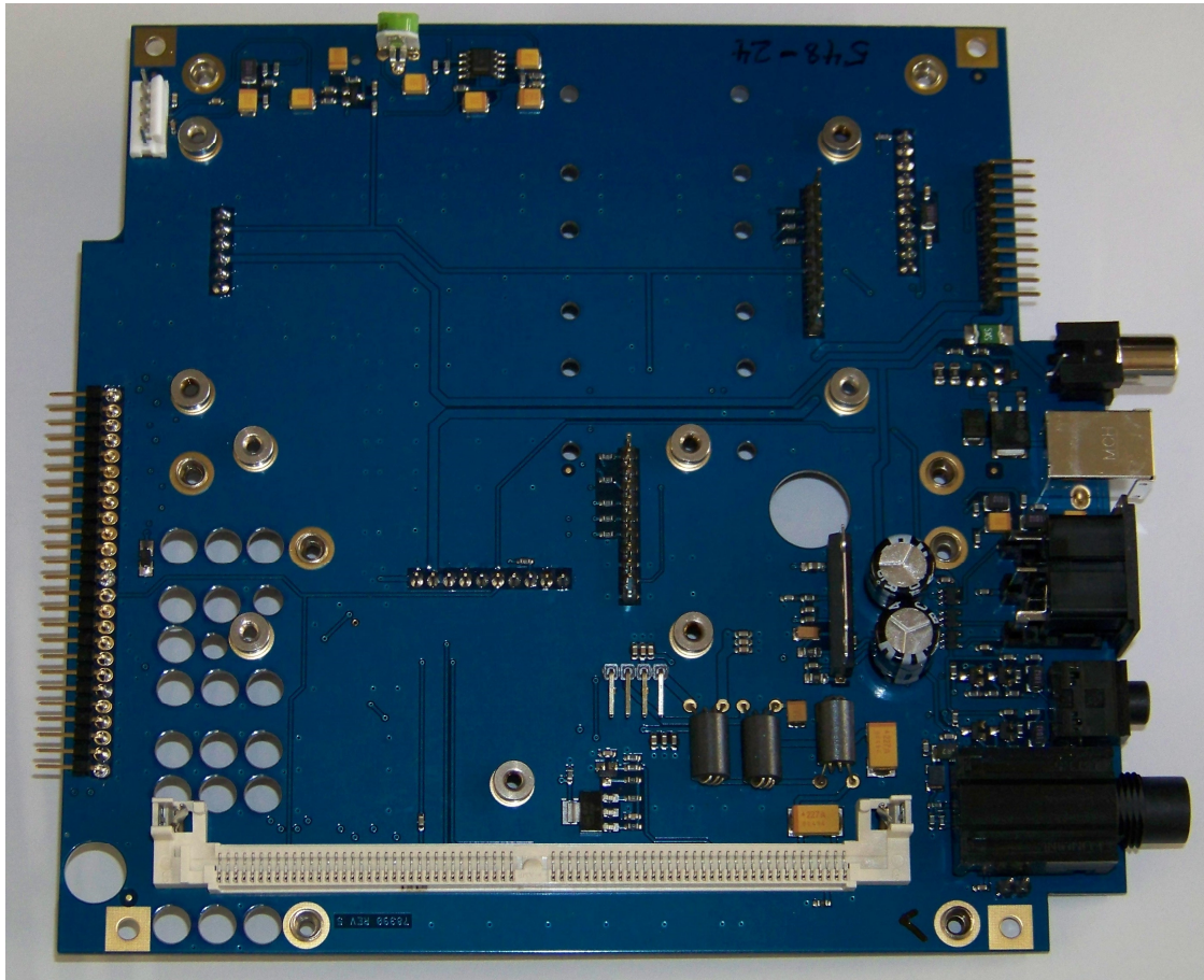
MOTHERBOARD TOP
