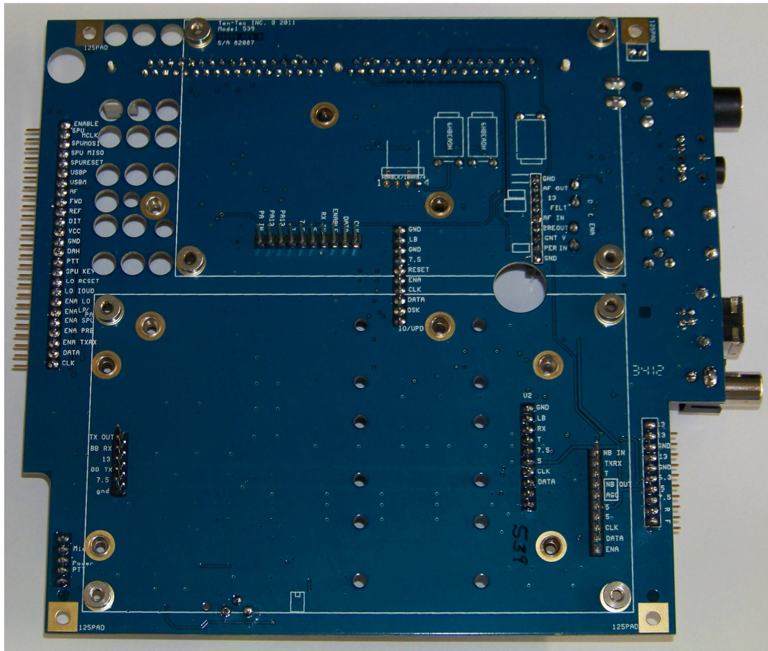
MOTHERBOARD BOTTOM
