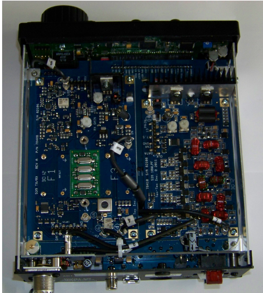
TOP VIEW (W/O FILTER COVER)
