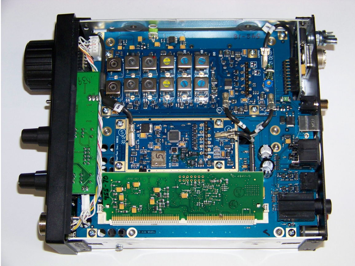
BOTTOM VIEW
