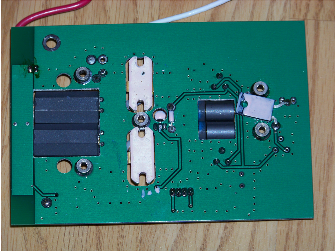
78401 REV B AMPLIFIER BOARD (BOTTOM VIEW)
