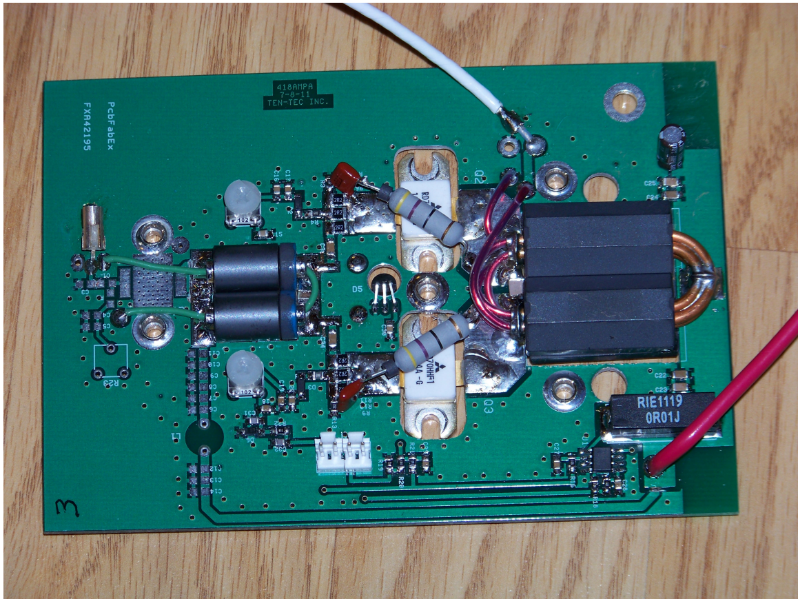
78401 REV B AMPLIFIER BOARD (TOP VIEW)
