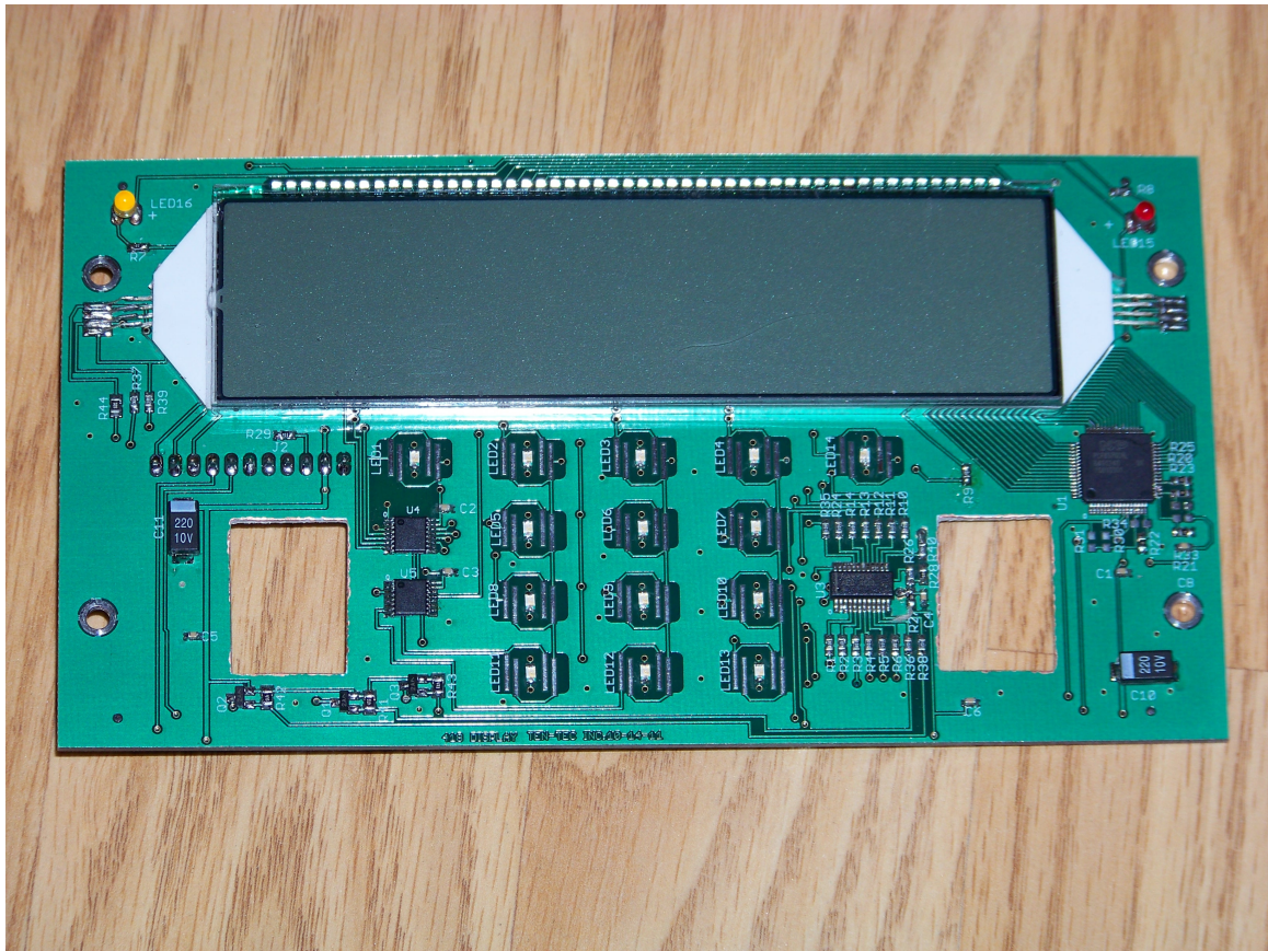
78400 REV C DISPLAY BOARD (TOP VIEW)
