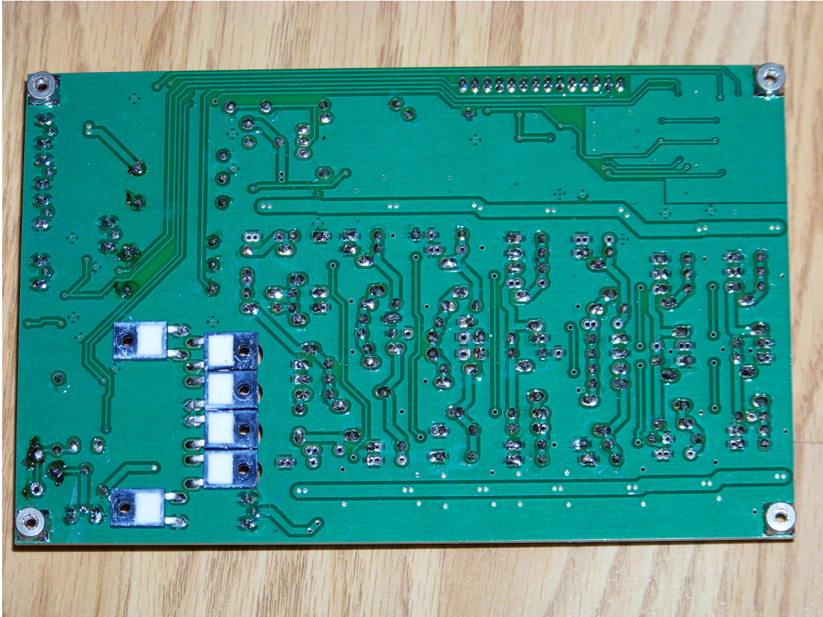
78399 REV B LOWPASS FILTER BOARD (BOTTOM VIEW)
