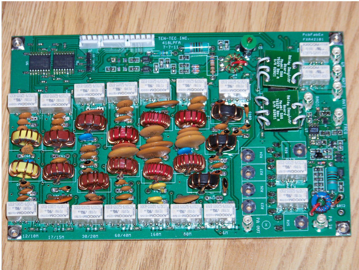
78399 REV B LOWPASS FILTER BOARD (TOP VIEW)
