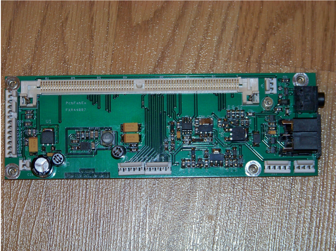
78398 REV C MOTHERBOARD (TOP VIEW)
