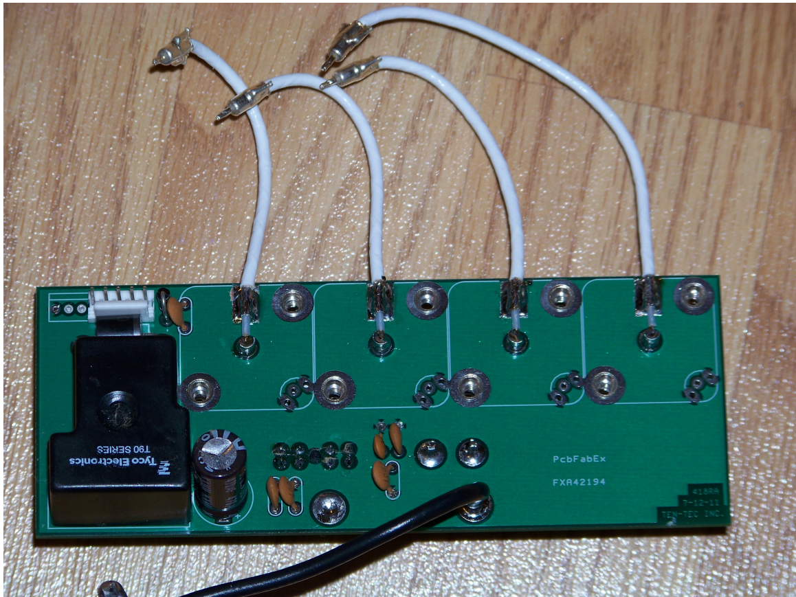
78397 REV B REAR PANEL BOARD (BOTTOM VIEW)
