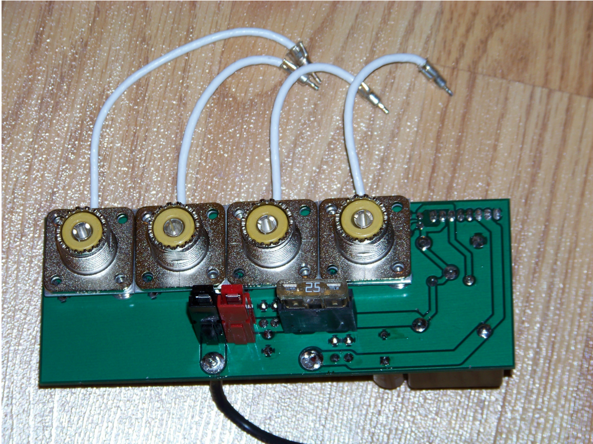
78397 REV B REAR PANEL BOARD (TOP VIEW)
