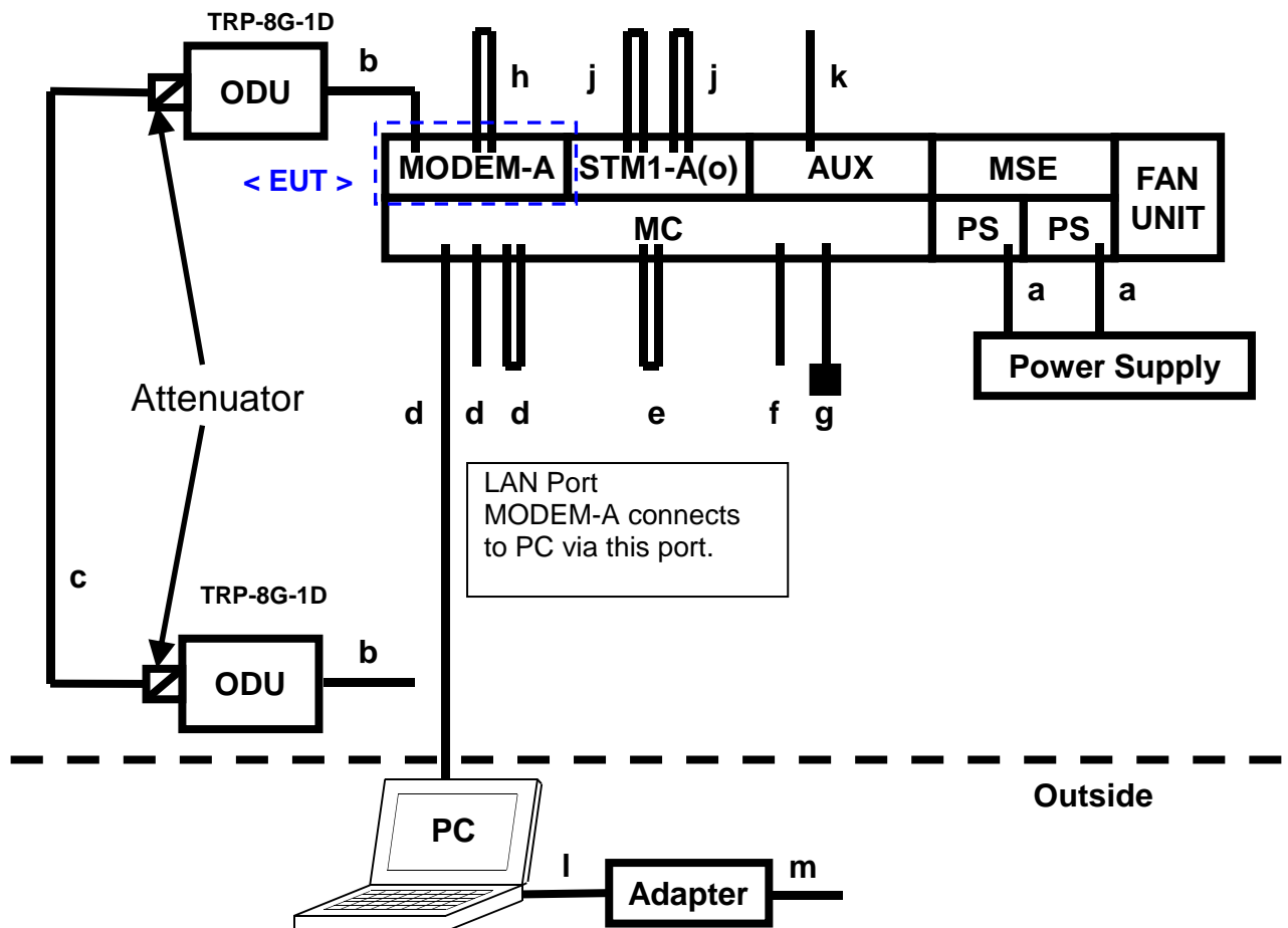
Figure 1-1 System Configuration Diagram
