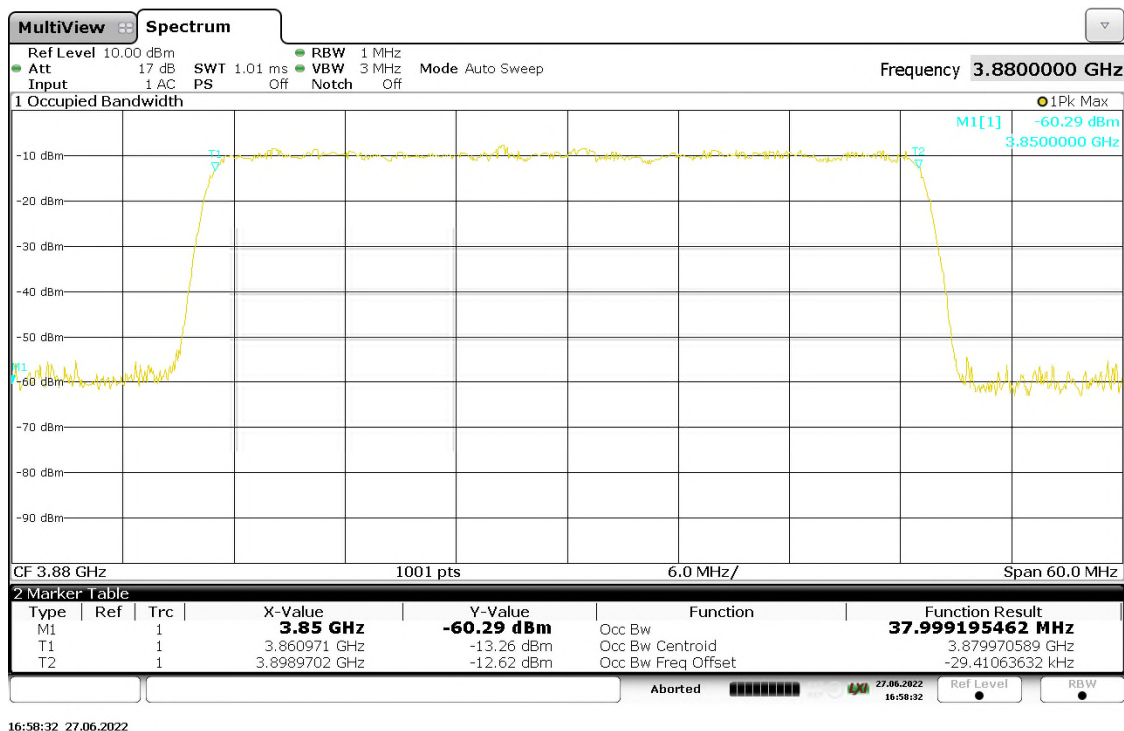
Figure 71: 99% Occupied Bandwidth, 1cc-1 (OBW=40MHz), 64QAM_TM3.1, High Channel, TX Port 25
