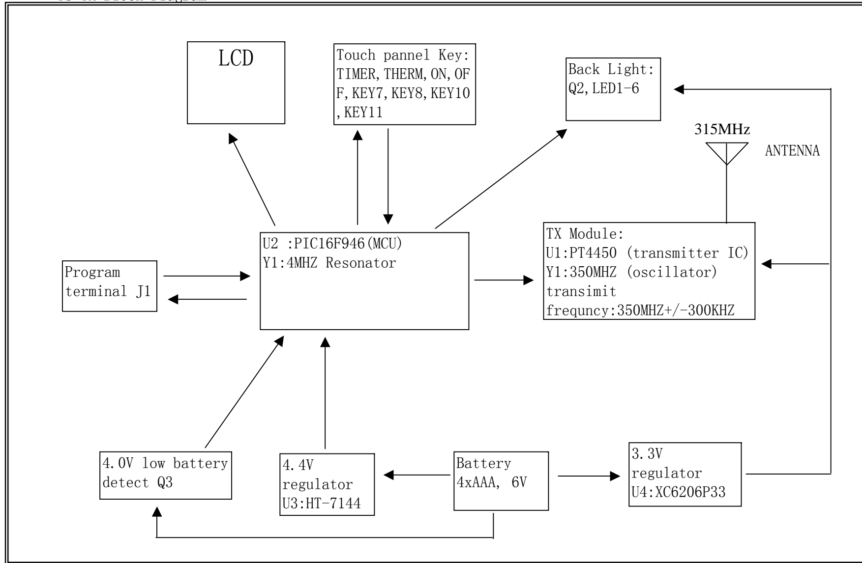
TS-TX Block Diagram
