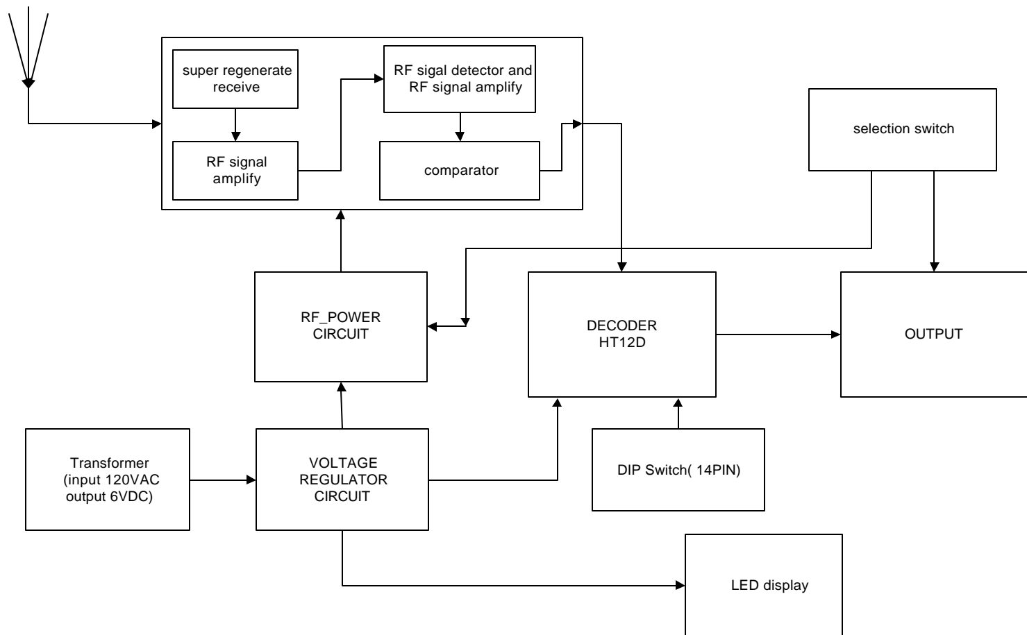
RF 350MHz receiver circuit
