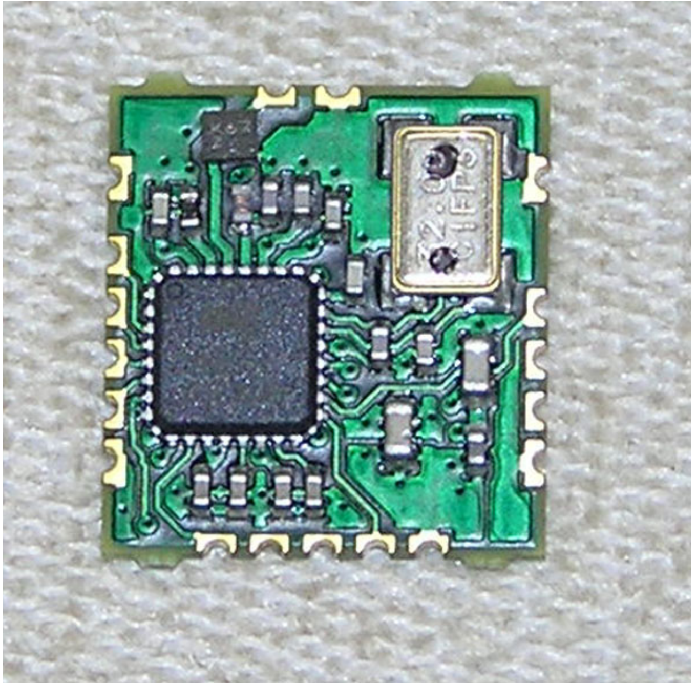
HA20 RF MODULE PCB ZM3102N FRONT
