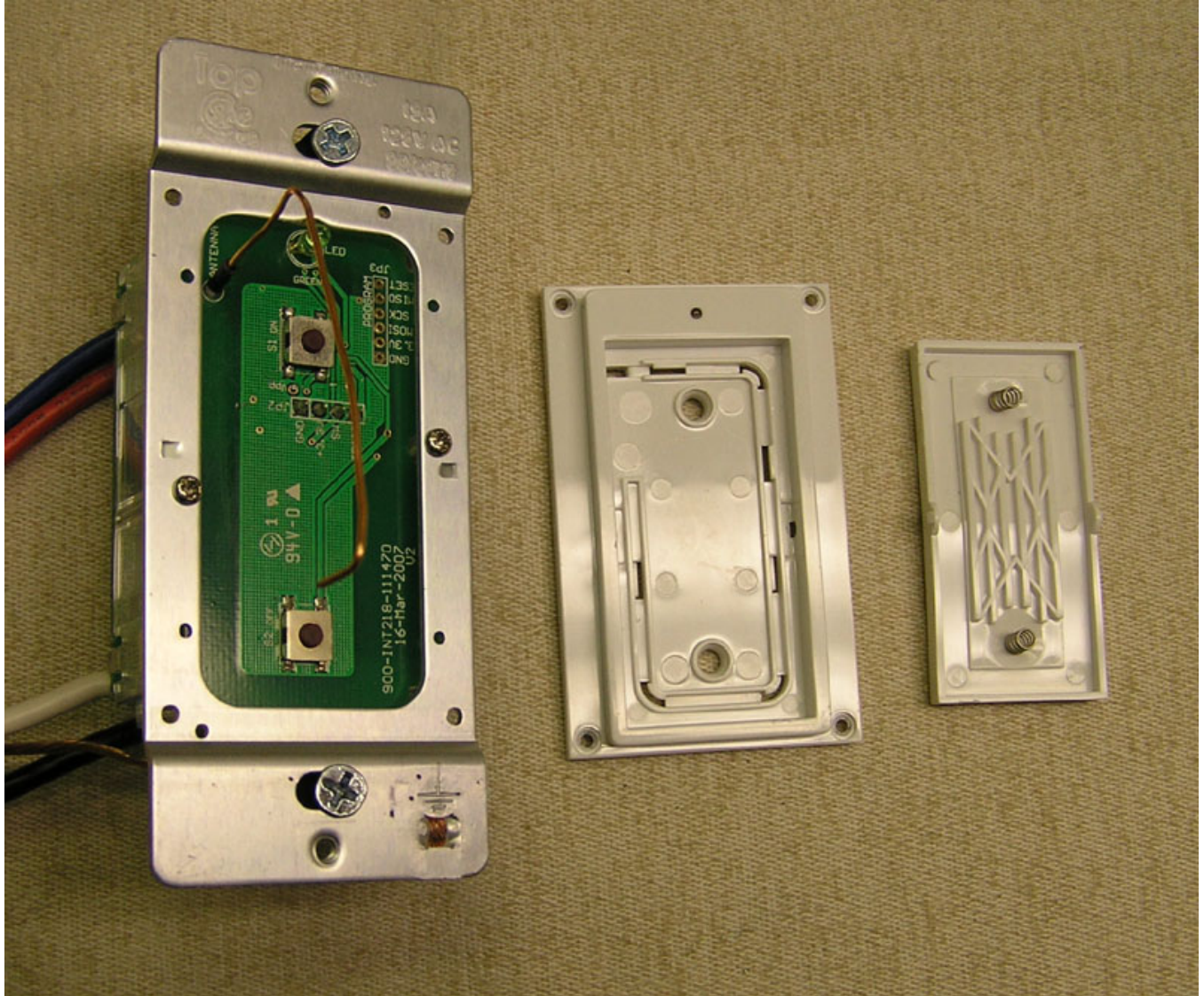
HA18 FRONT HOUSING REMOVED SHOWING BUTTON PCB
