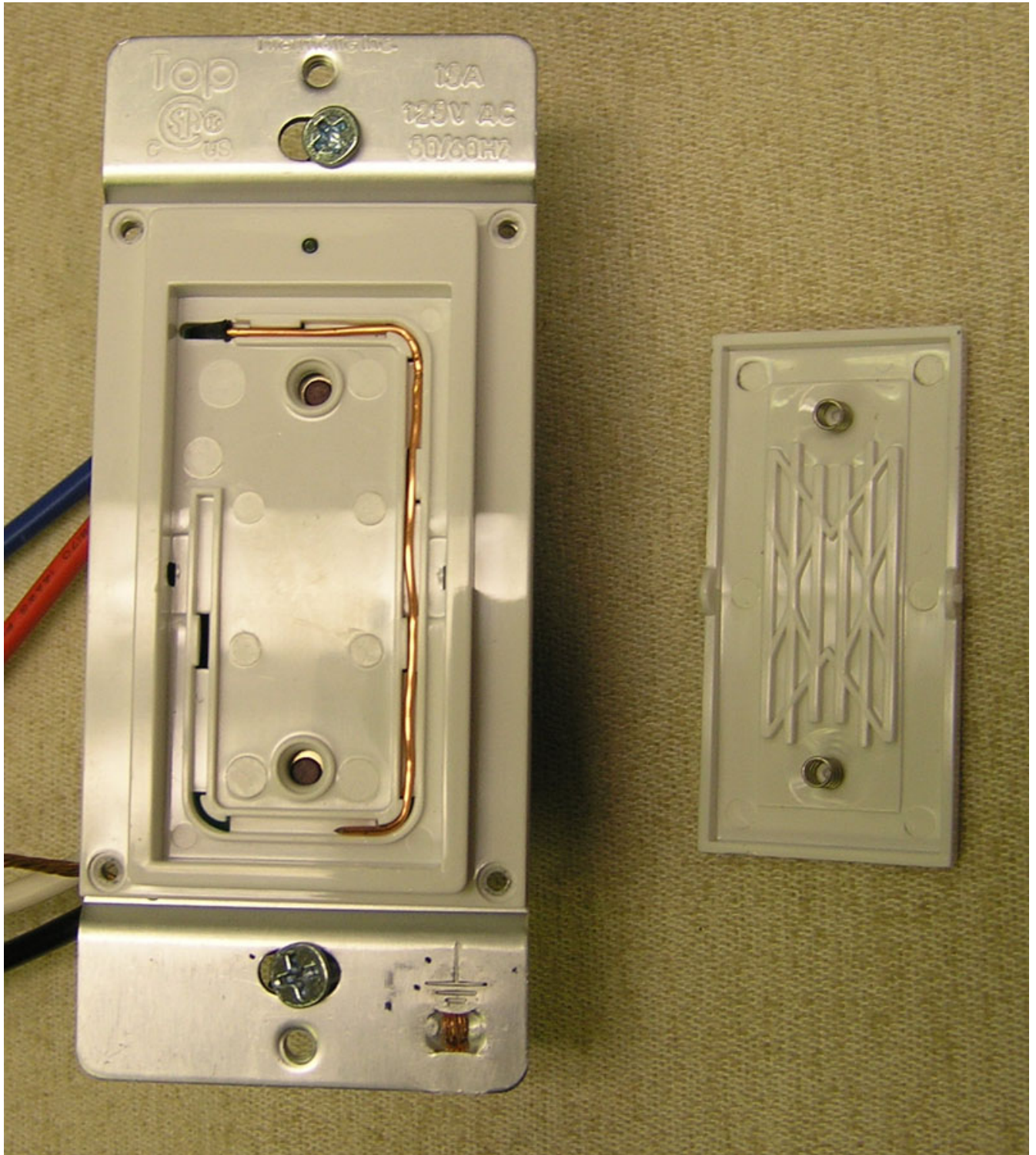
HA18 ROCKER PLATE REMOVED SHOWING ANTENNA
