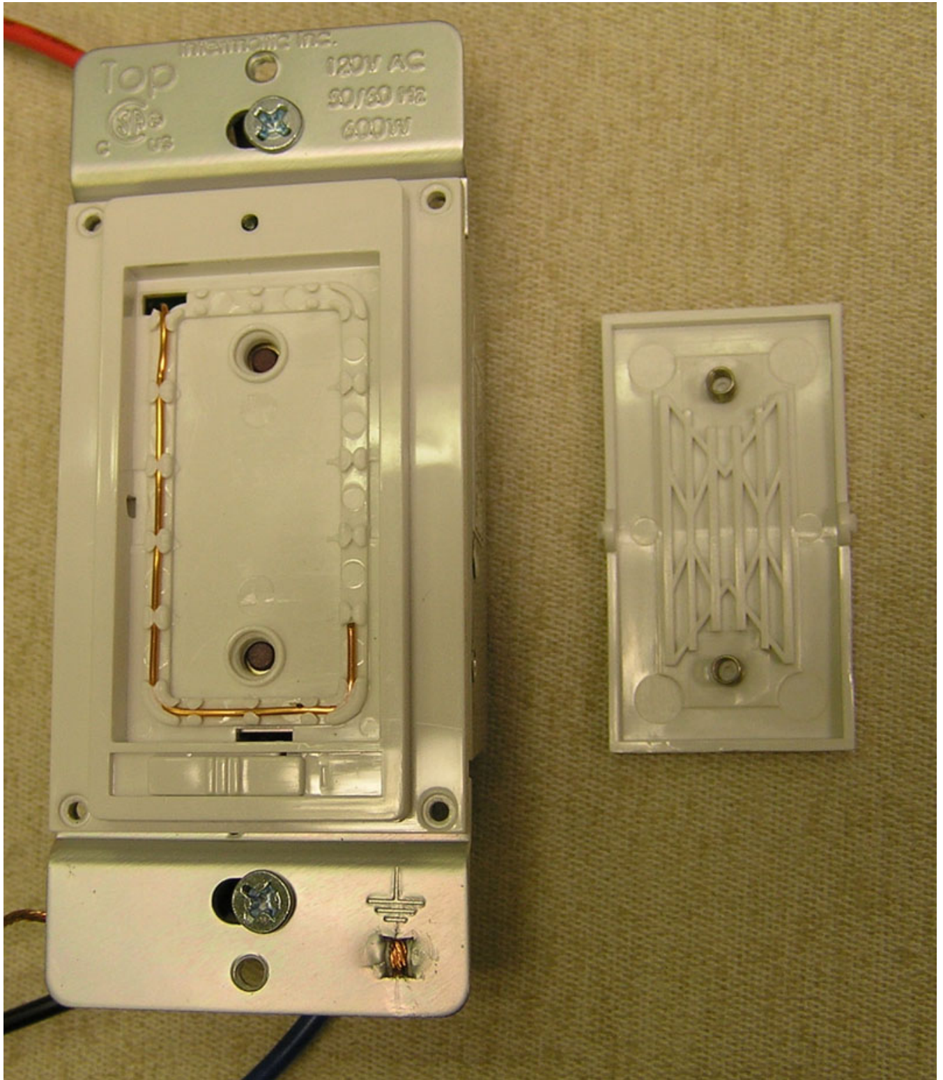
HA14 ROCKER PLATE REMOVED SHOWING ANTENNA
