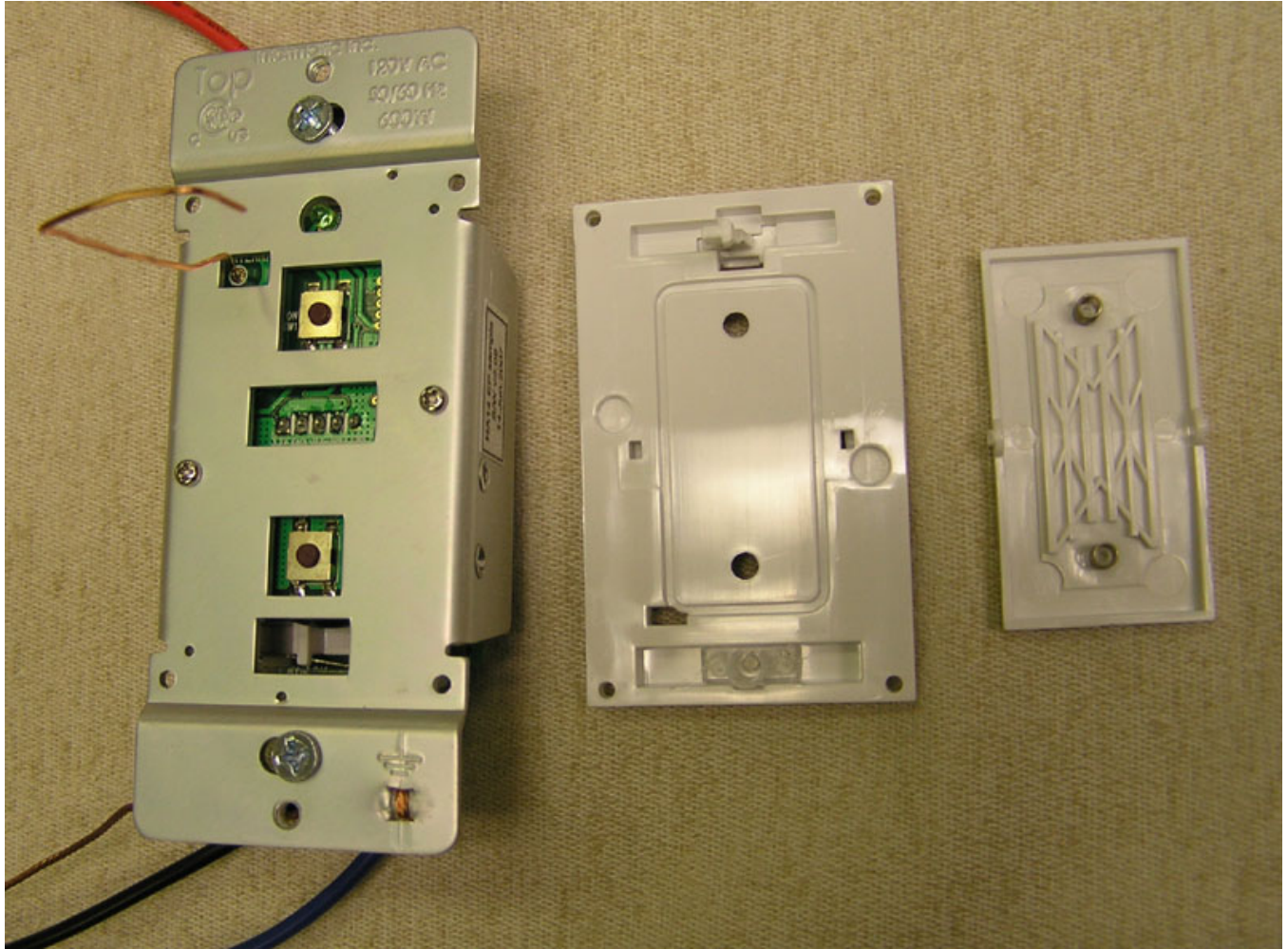
HA14 FRONT PLASTIC HOUSING REMOVED
