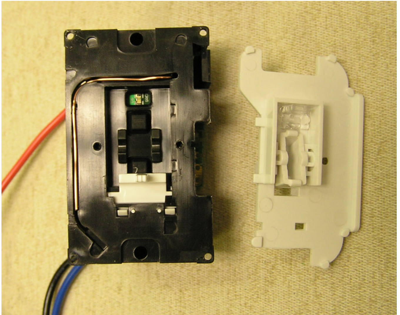
HA20 FRONT PLASTIC COVER REMOVED SHOWING ANTENNA
