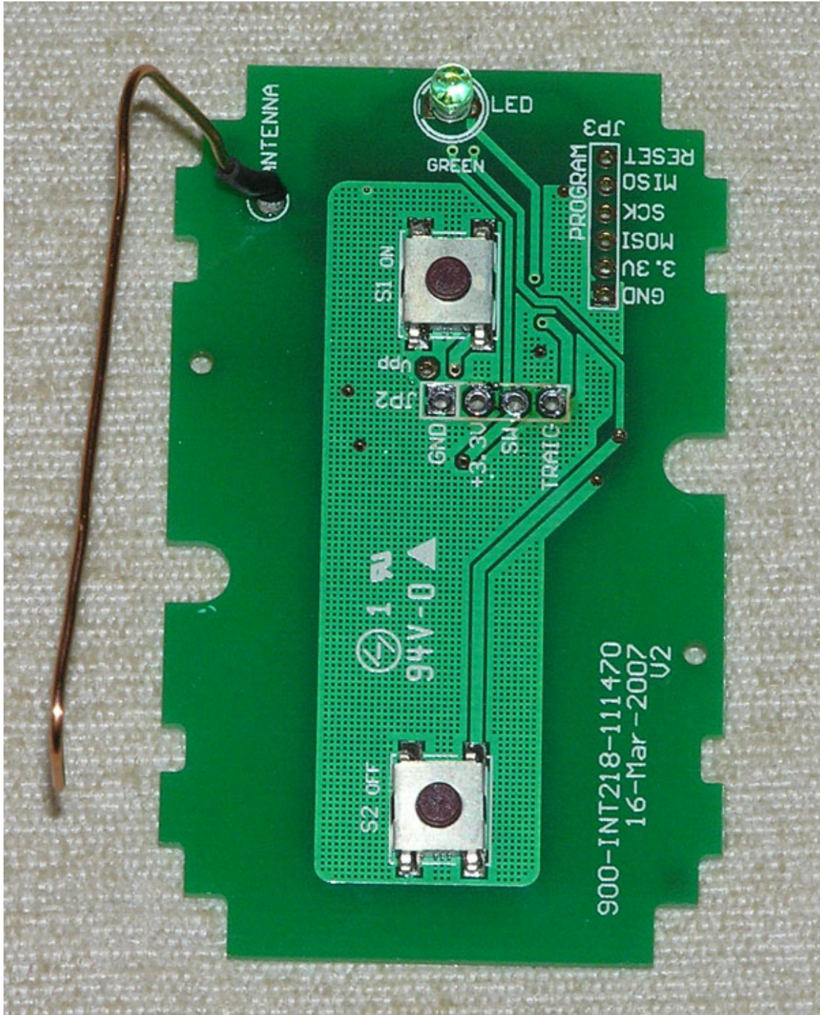
HA18 BUTTON PCB TOP
