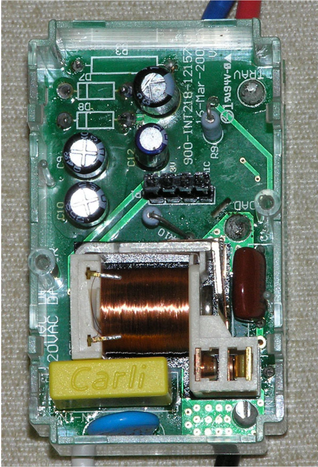
HA18 POWER PCB TOP
