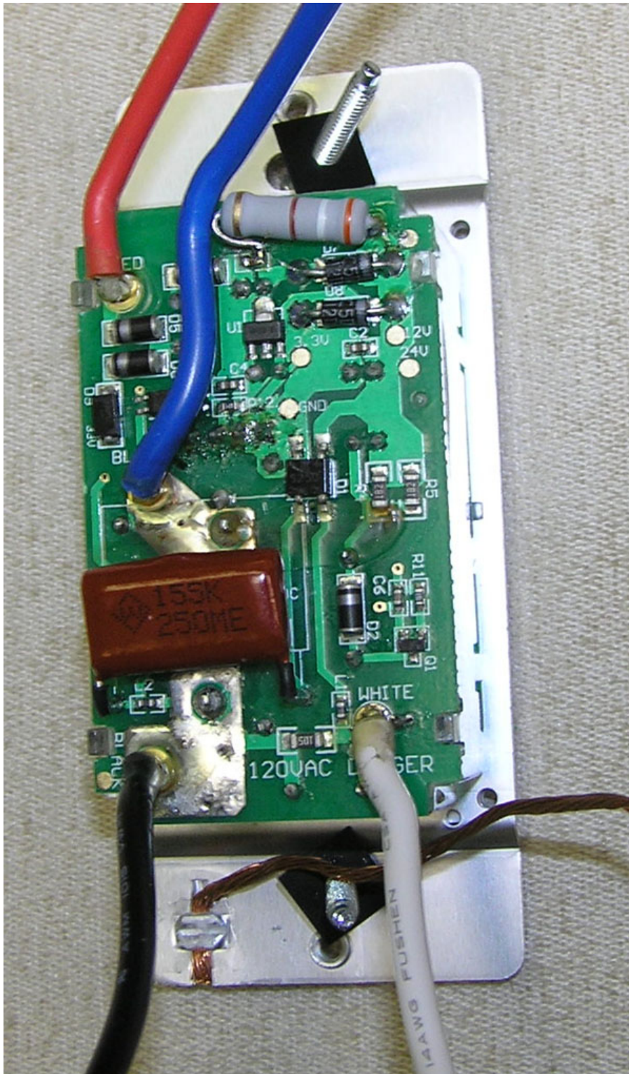
HA18 REAR PLASTIC HOUSING REMOVED
