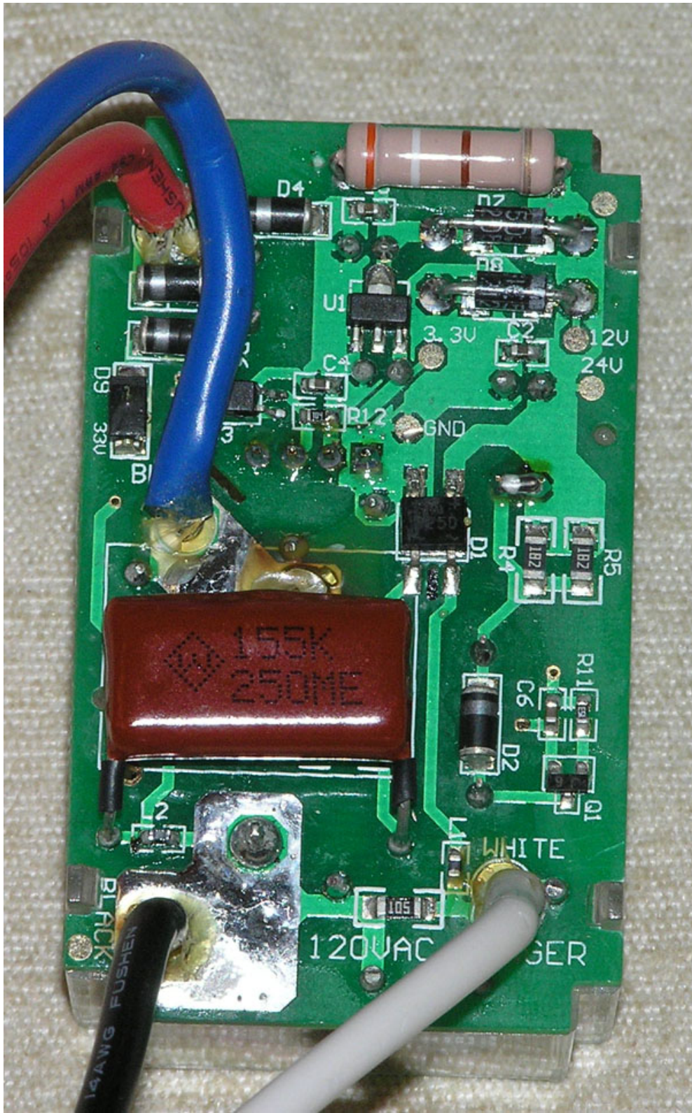
HA18 POWER PCB BOTTOM
