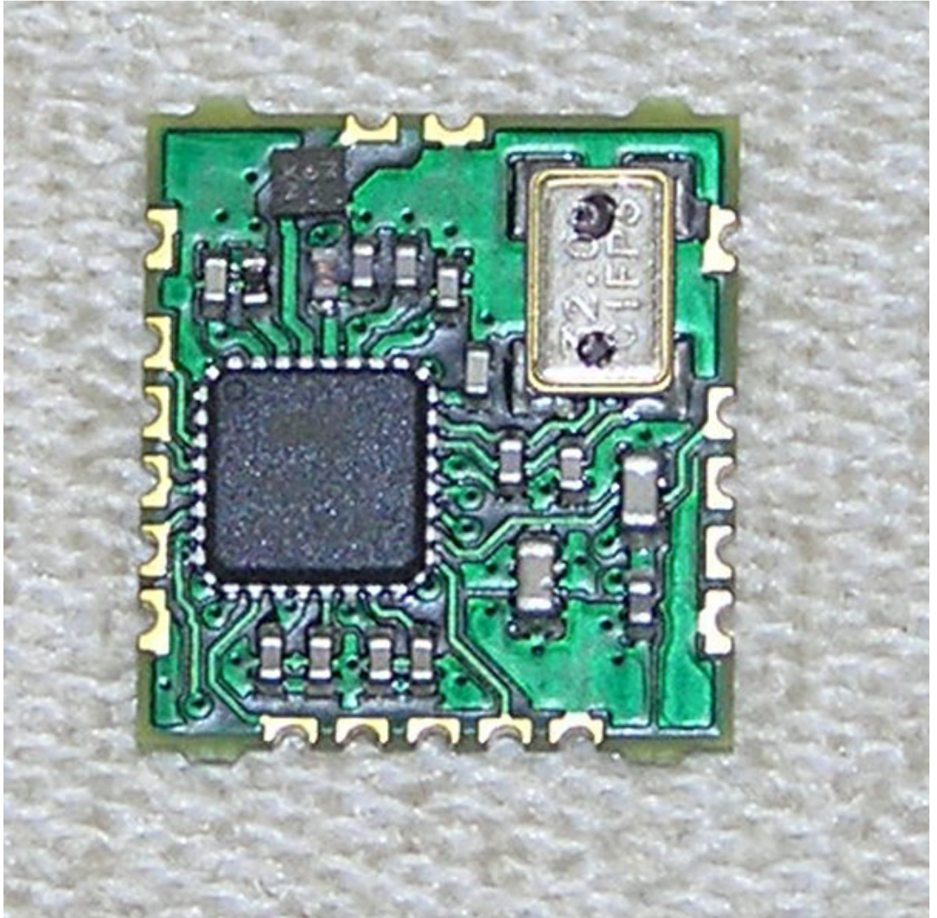
HA14 RF MODULE PCB ZM3102N FRONT
