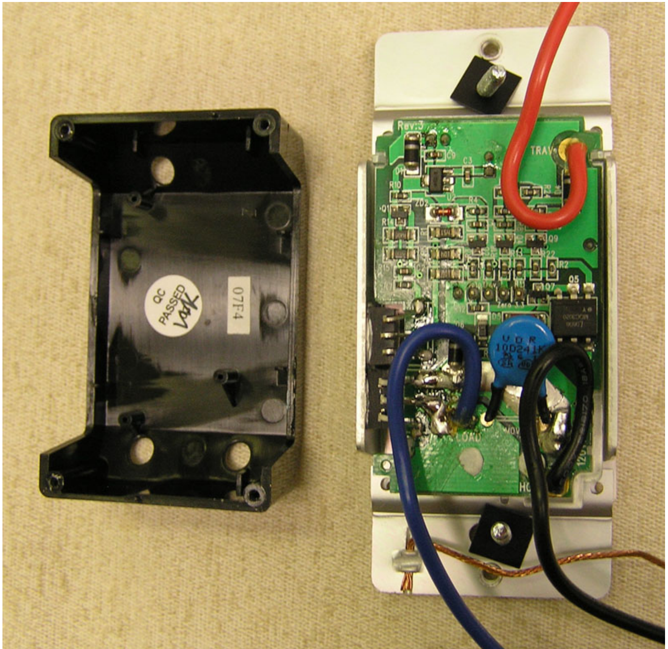
HA14 REAR PLASTIC HOUSING REMOVED
