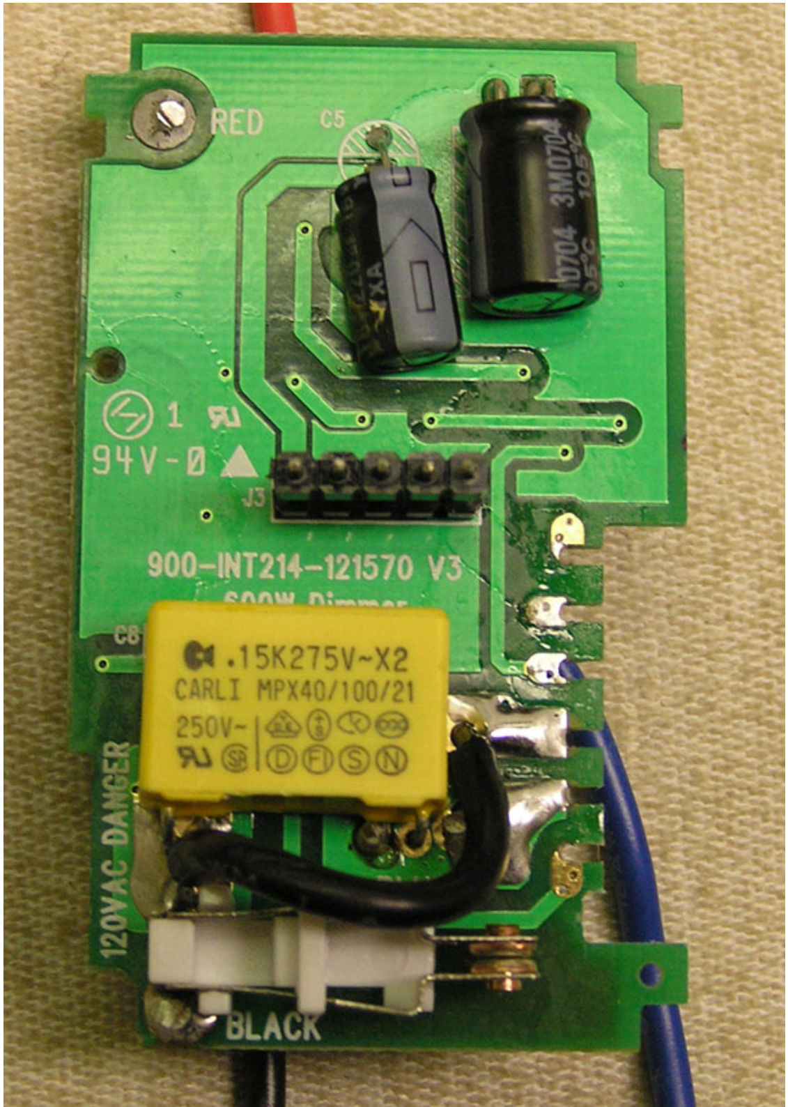
HA14 POWER PCB TOP
