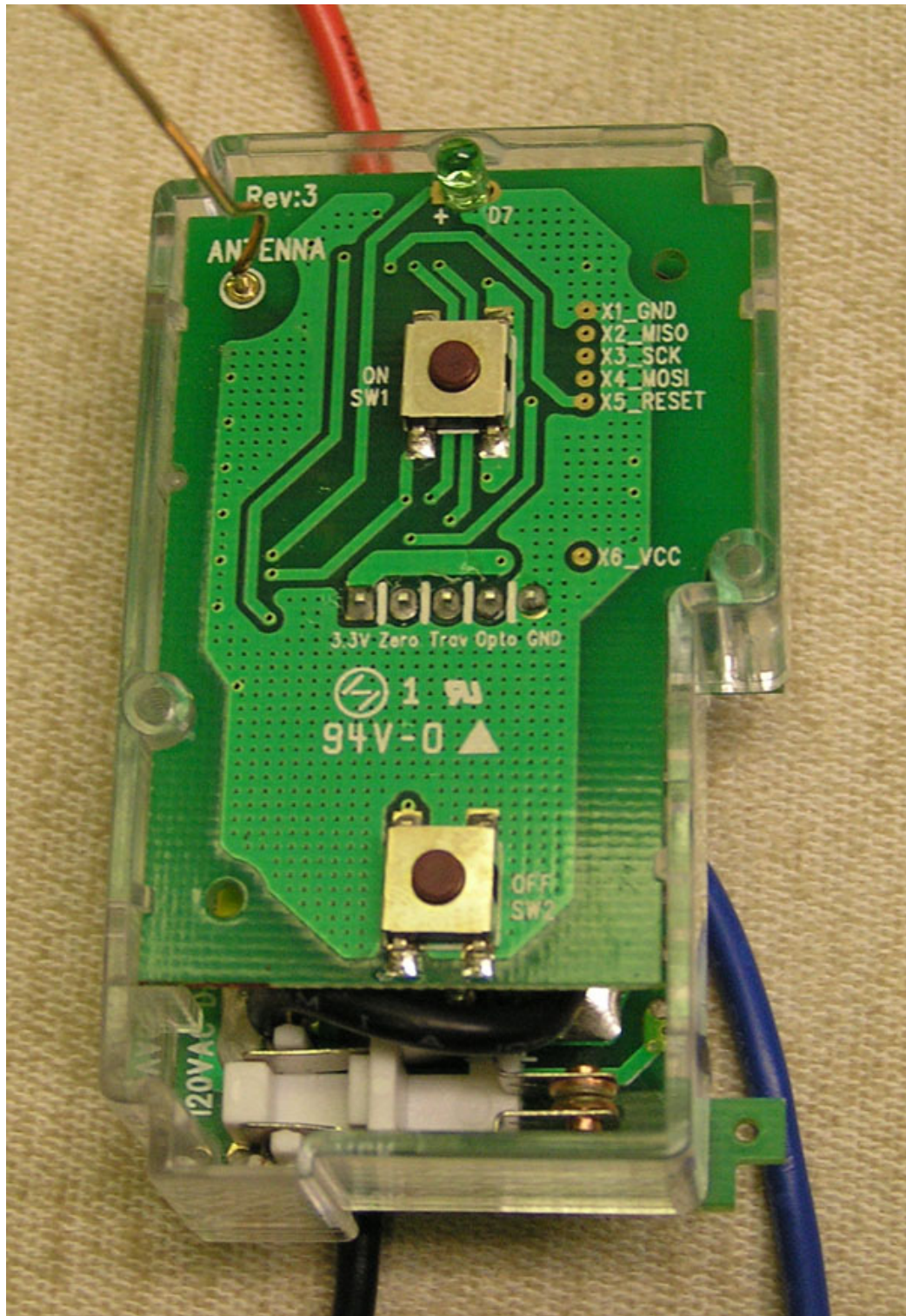
HA14 KEY PCB TOP
