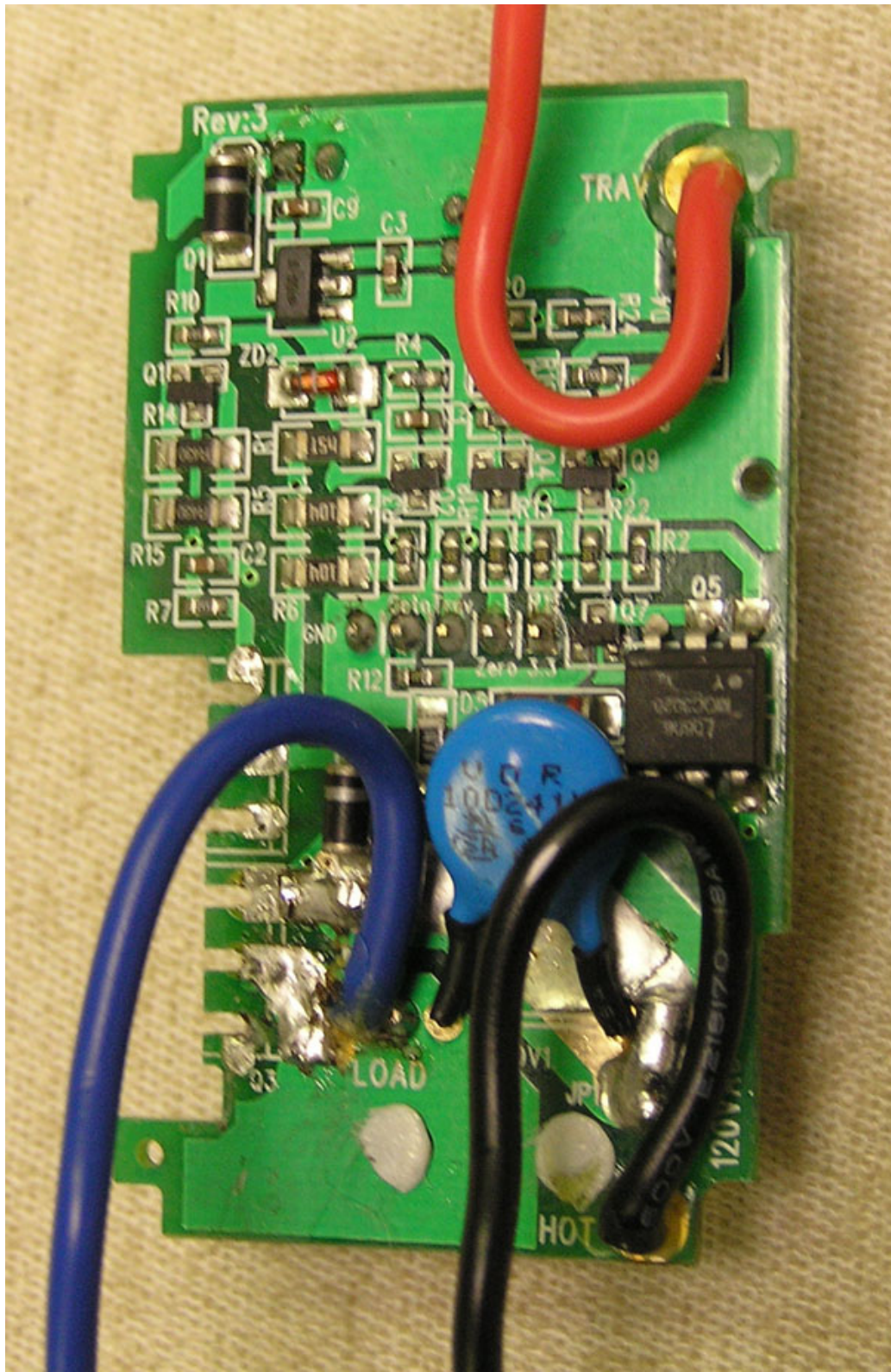
HA14 POWER PCB BOTTOM
