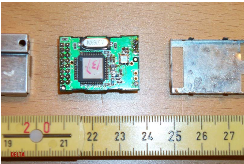
Photo 4 RF Module. Screens removed. ASIC side of module
