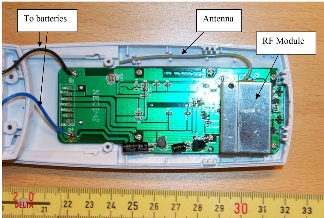
Photo 1 Base print with RF Module. Component side
