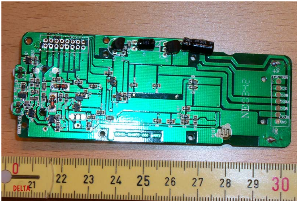
Photo 3 Base print. RF Module removed
