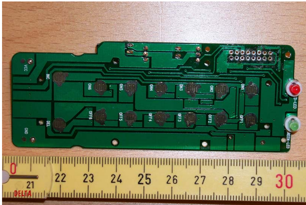
Photo 2 Base print. Component side down.
