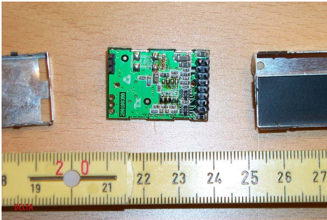
Photo 5 RF Module. Screens removed. ASIC side down.
