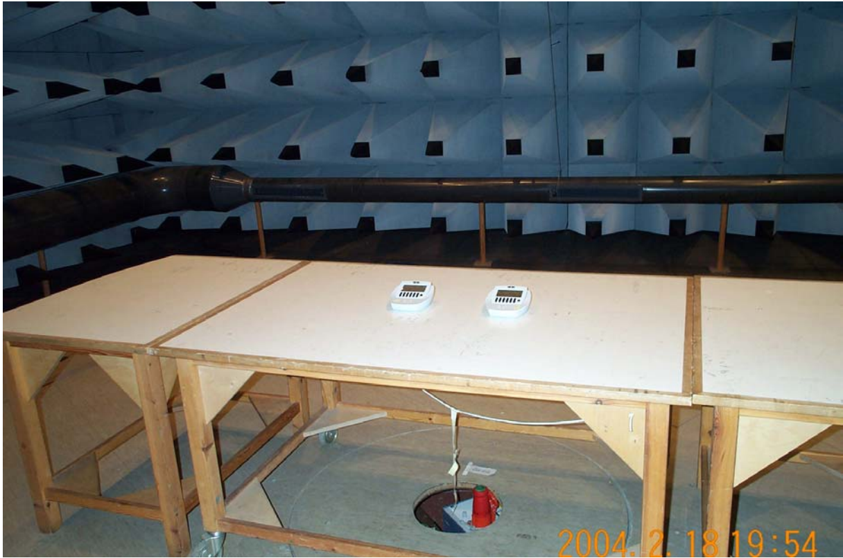
Photo 1 Set-up for emission measurements. Constant TX CW unit and constant Rx unit.
