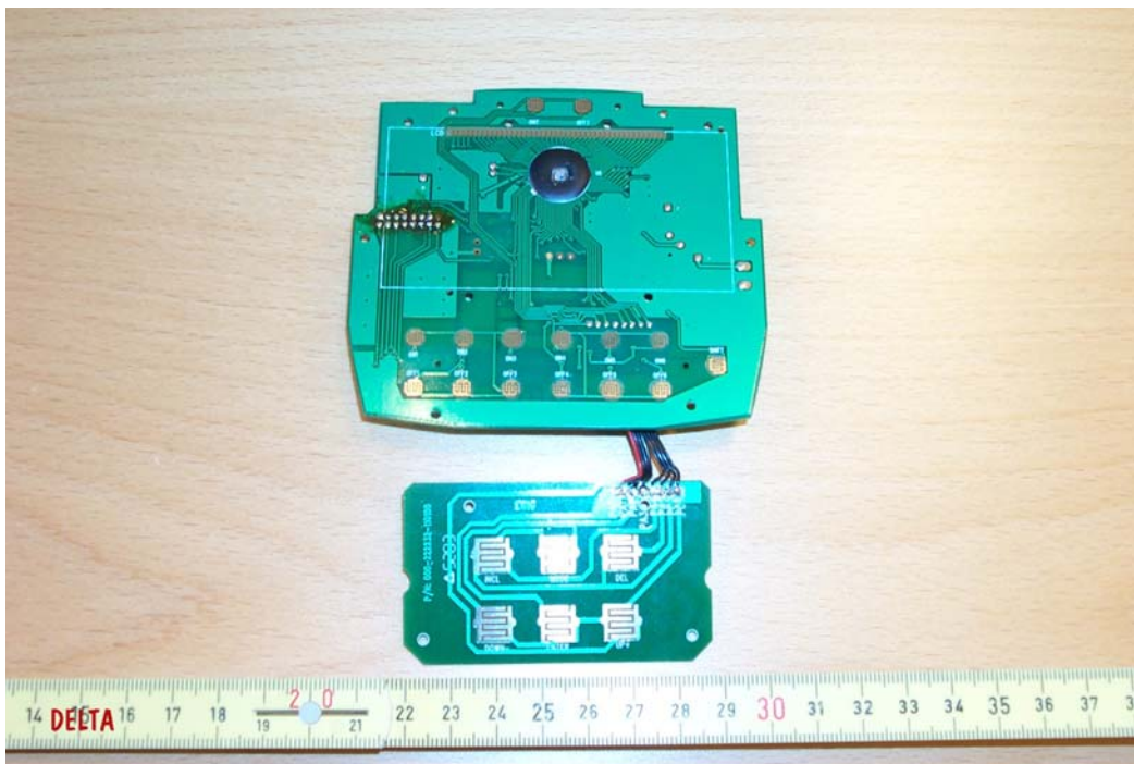
Photo 4 As photo 3 but with LCD display removed.
