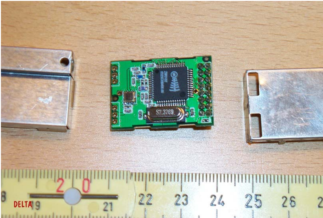
Photo 5 RF Module. ASIC side. Screens removed.
