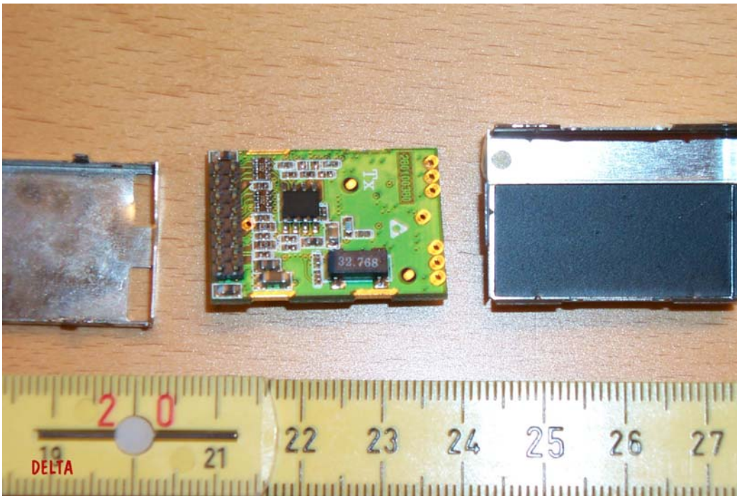
Photo 6 RF Module. ASIC side down. Screens removed.
