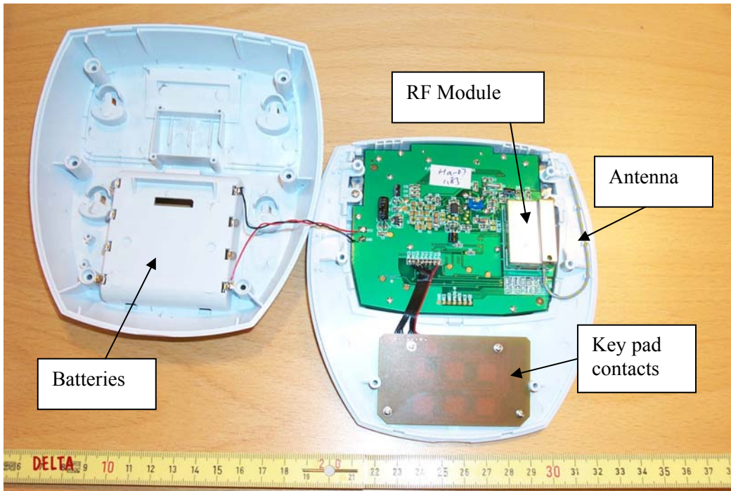
Photo 1 Main board. Component side.
