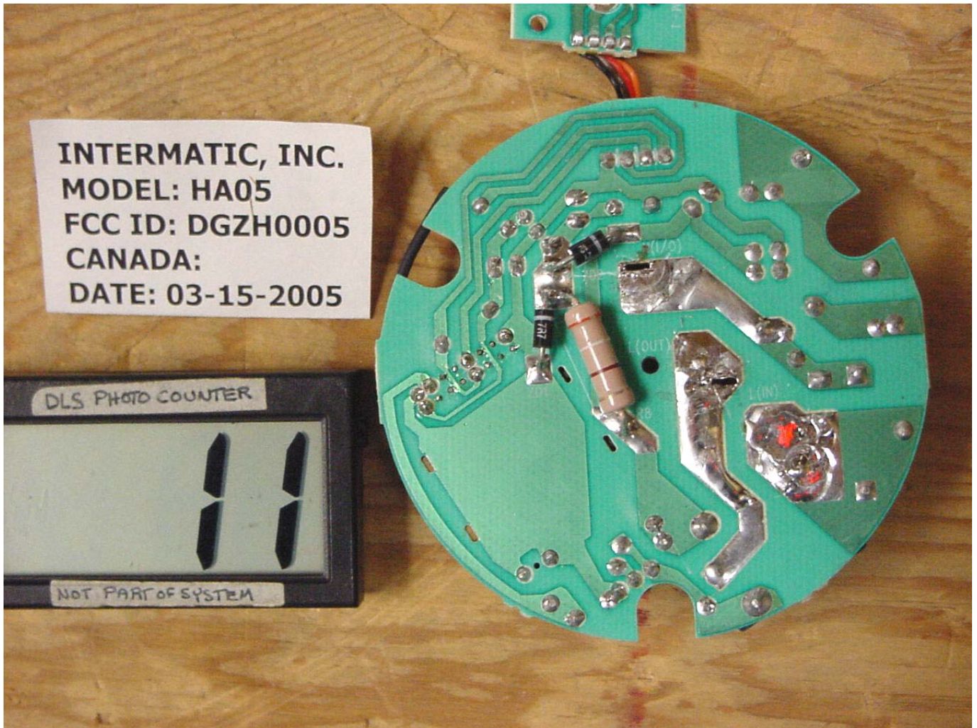
Circuit Board Solder Side
