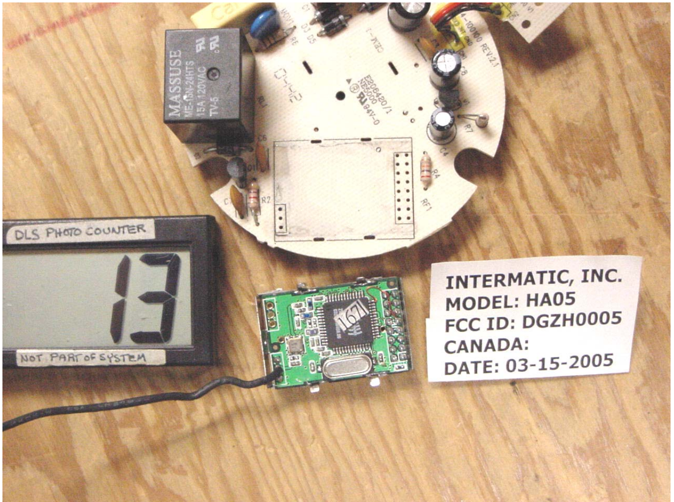
RF BOARD REMOVED
