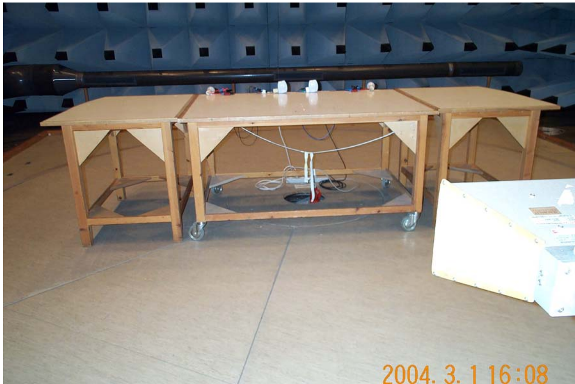
Photo 4 Measurement set-up > 1 GHz.
