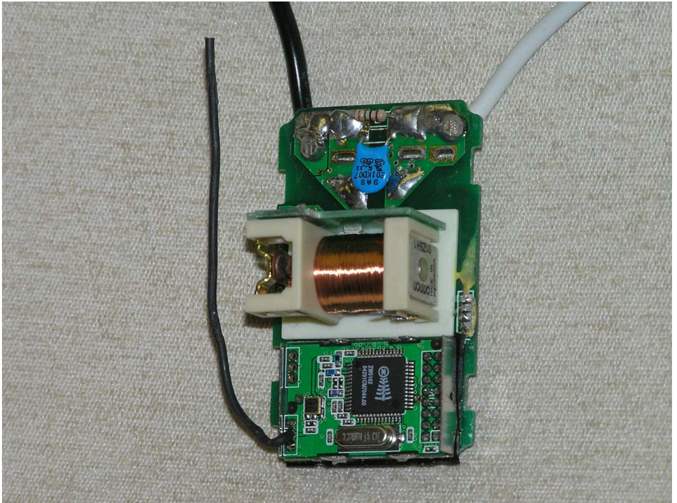
MOUNTED Z-WAVE MODULE / SHIELD REMOVED
