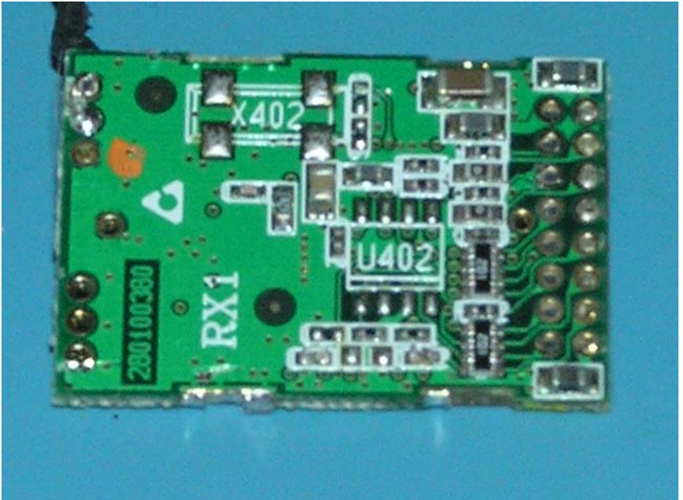
BOTTOM SIDE Z-WAVE MODULE WITHOUT SHIELD
