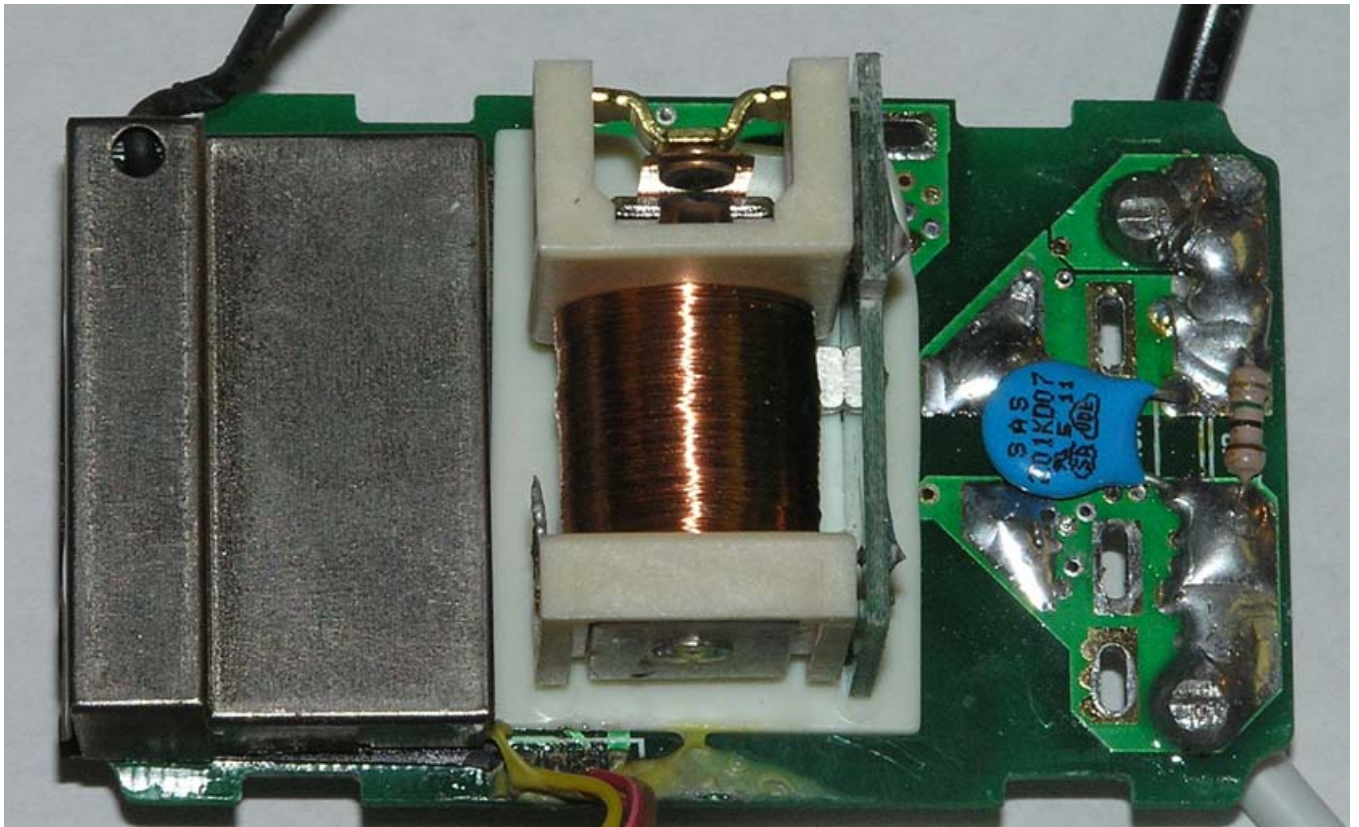
INSIDE REAR
