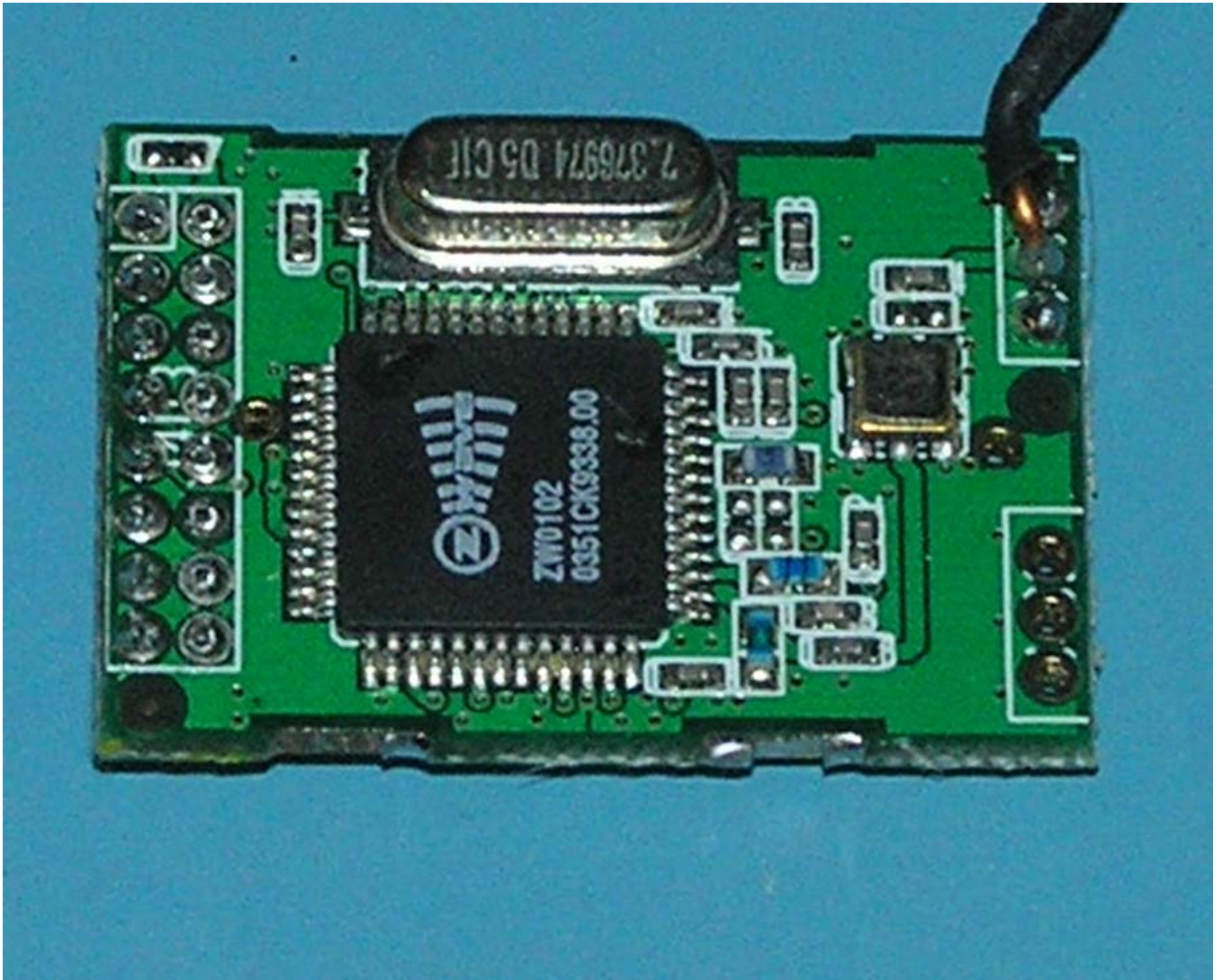
TOP SIDE Z-WAVE MODULE WITHOUT SHIELD
