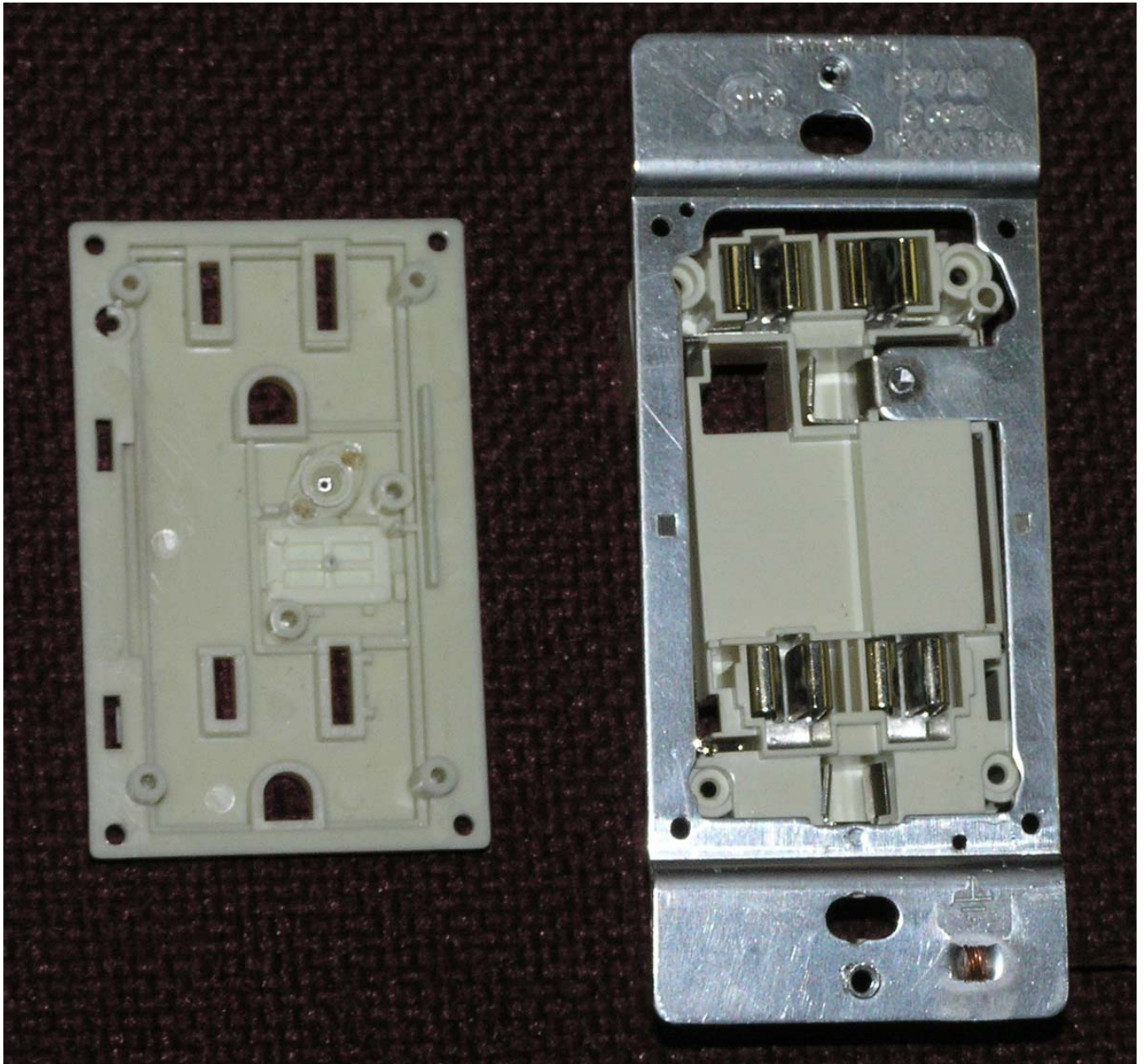
INSIDE FRONT
