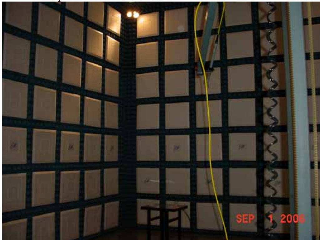
Test Setup for Radiated Emissions, 908MHz – Vertical Polarization
