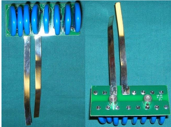
Tank Circuit Padder Caps
