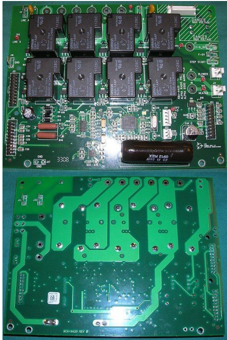
AC Input Switch Mains Board
