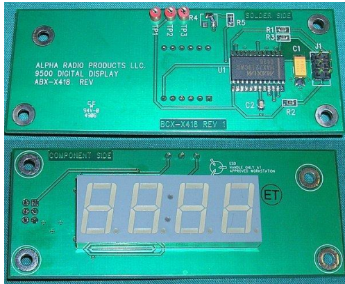
Digital Display Board
