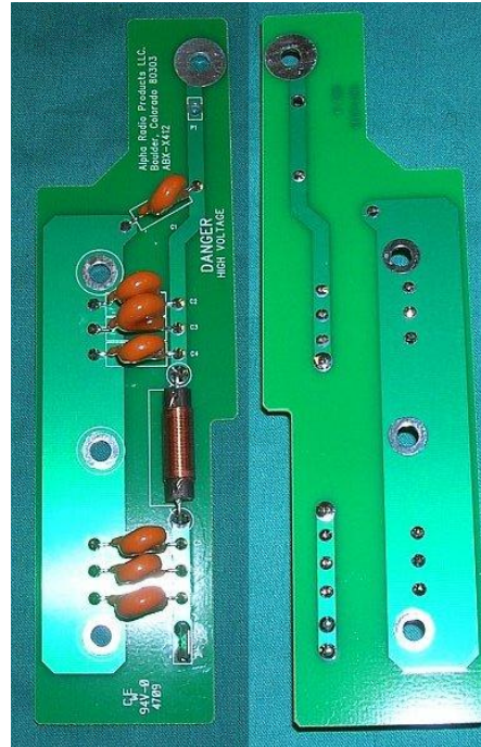
High Voltage Filter Board
