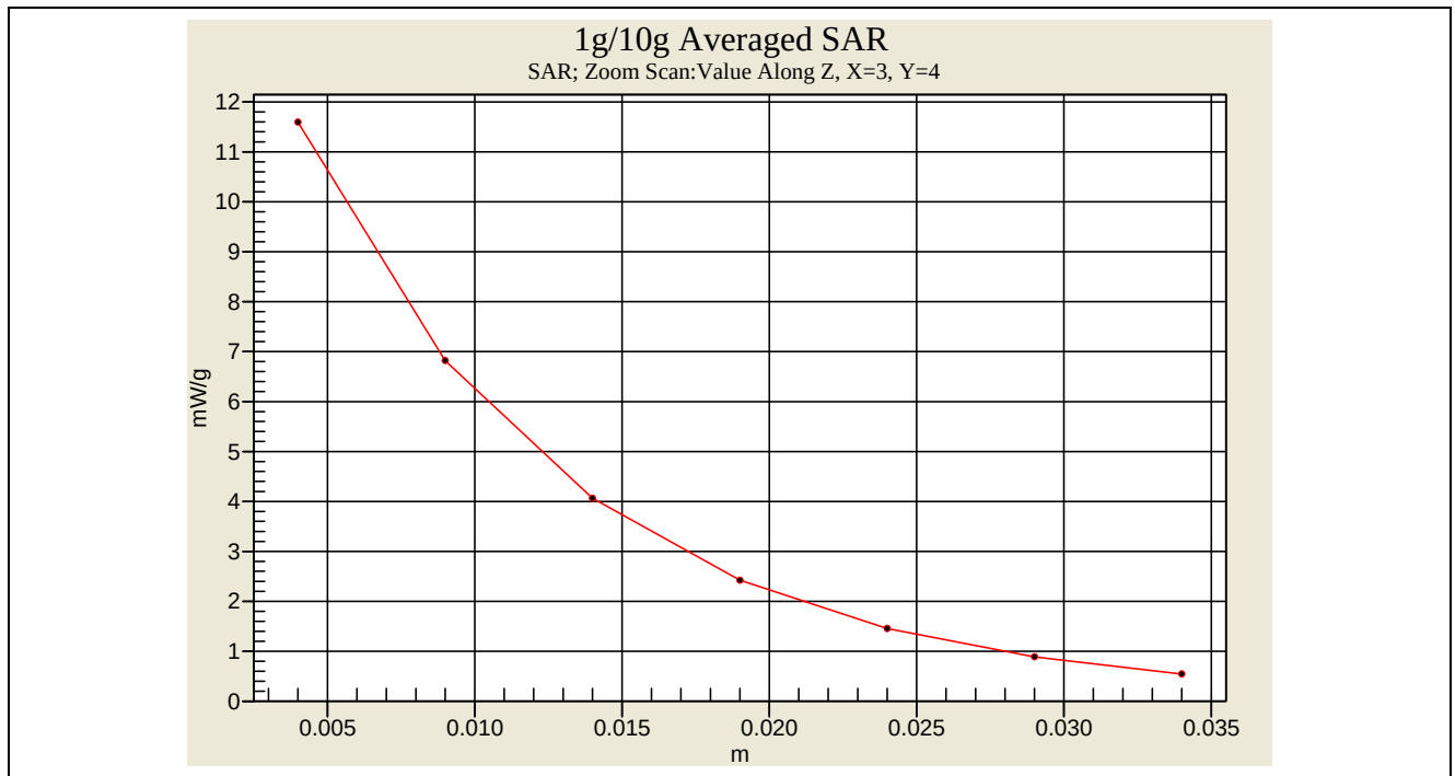
Body-Tissue-Simulating-Liquid 1950MHz ( 2008.07.21 )
