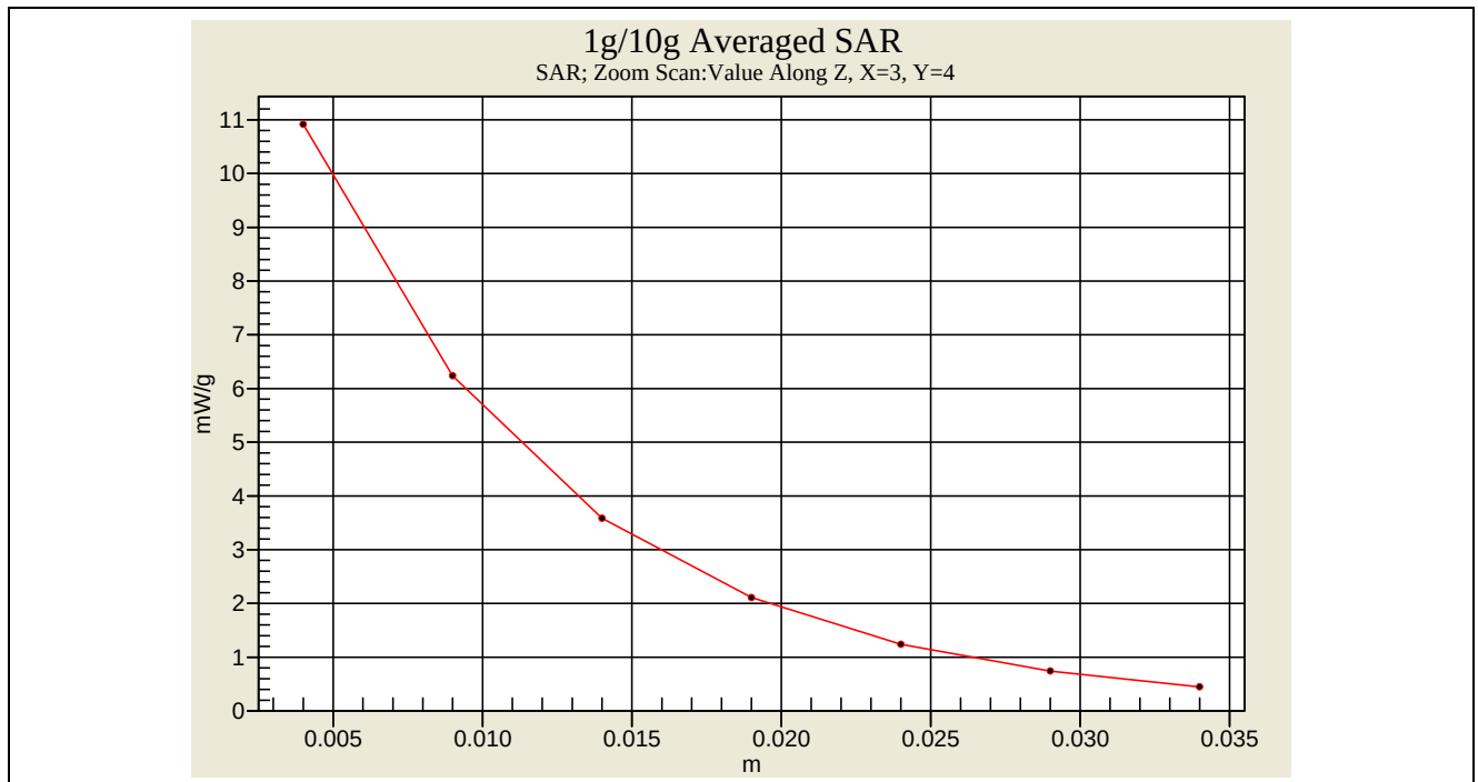
Head-Tissue-Simulating-Liquid 1950MHz ( 2008.11.07 )
