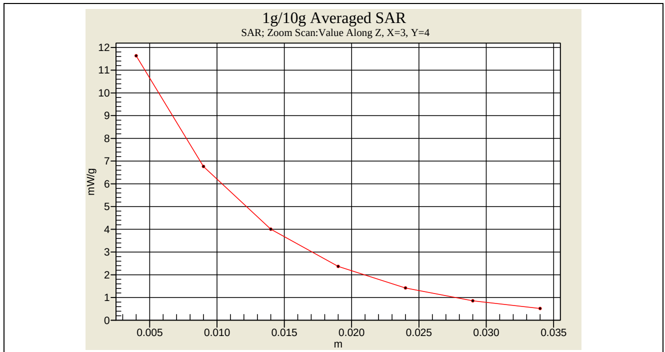
Body-Tissue-Simulating-Liquid 1950MHz ( 2008.09.04 )
