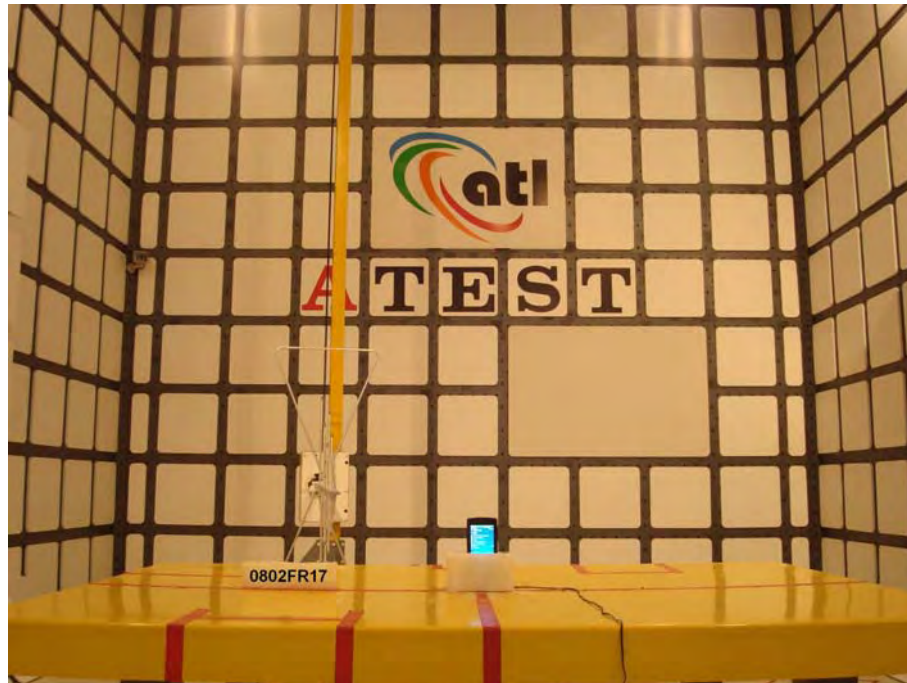
Figure 4. Front View of the Test Configuration
