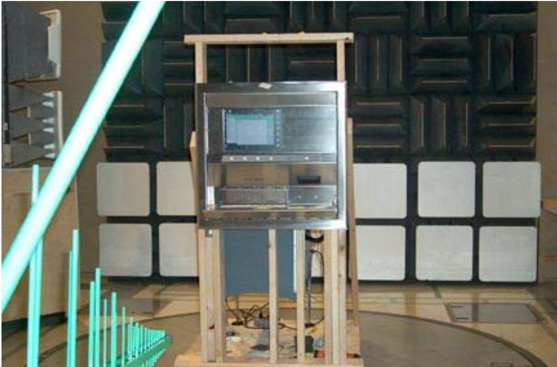
Radiated Emissions
