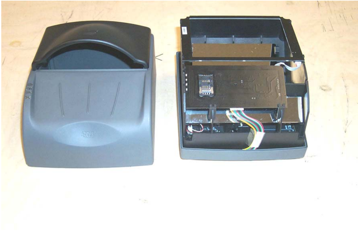
PV40 with cover removed
