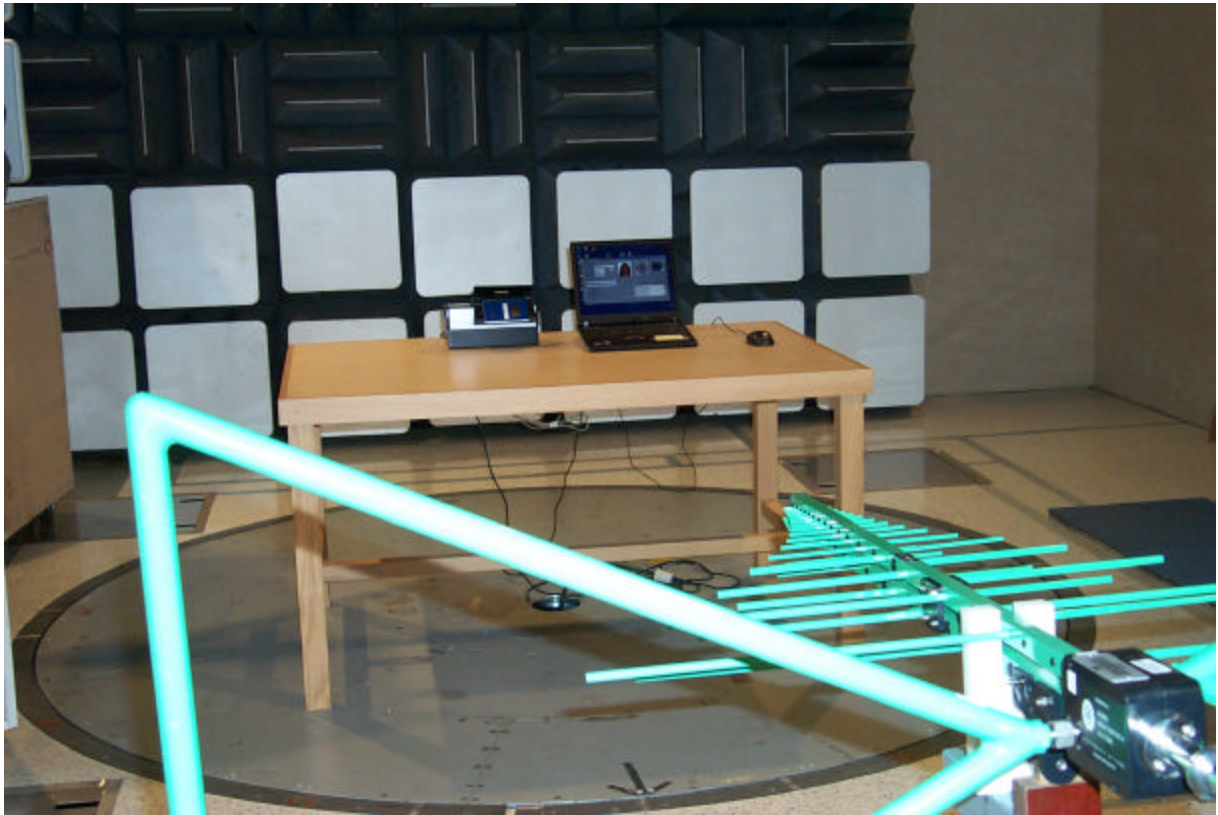
PV30 ACG 30 MHz to 1000 MHz
