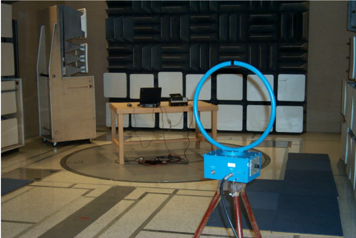
PV30 ACG 12 MHz to 30 MHz
