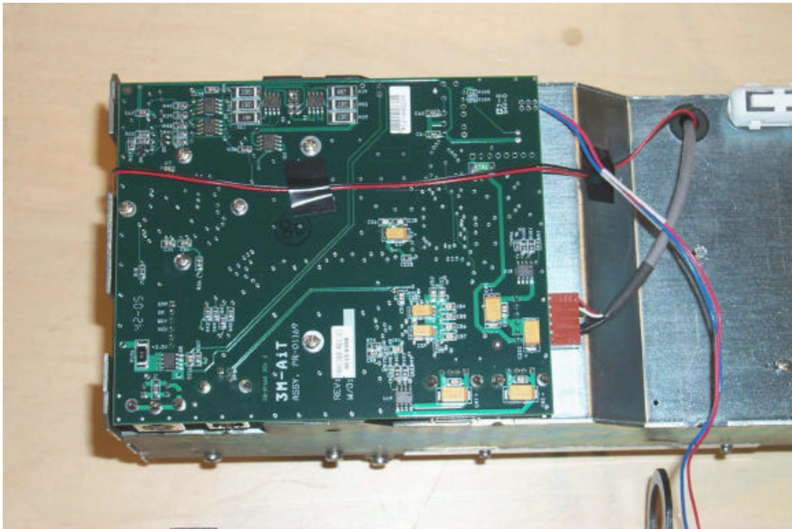
PV30 (ACG) CPU Board
