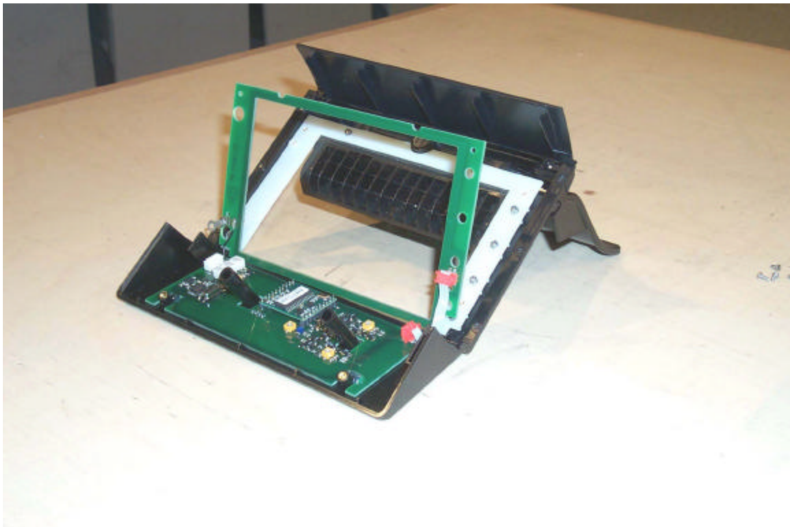
PV30 (ACG) Antenna Board (vertical board)
