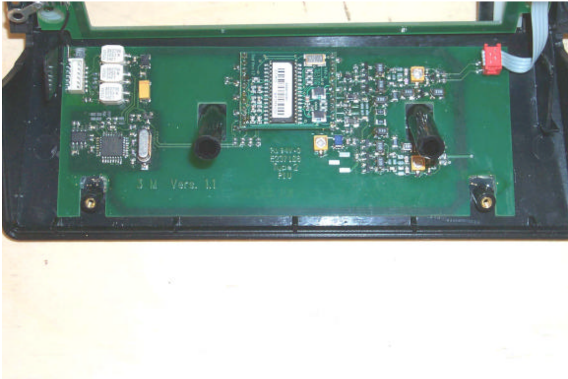
PV30 (ACG) RFID Reader Board
