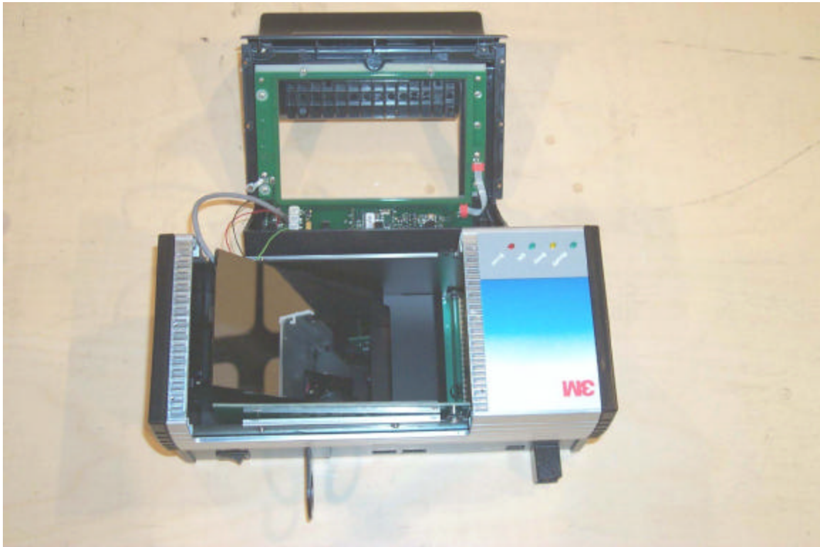
PV30 (ACG) RFID Antenna Board (top green board)
