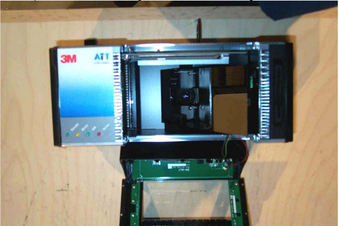
PV33 top frame removed showing internal antenna mounting
