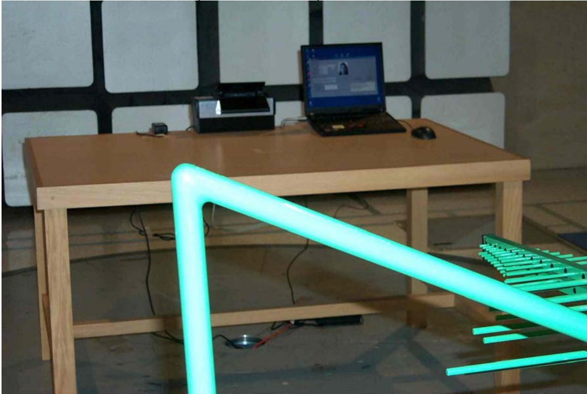
PV33 Radiated Emissions (1 GHz – 5 GHz)
