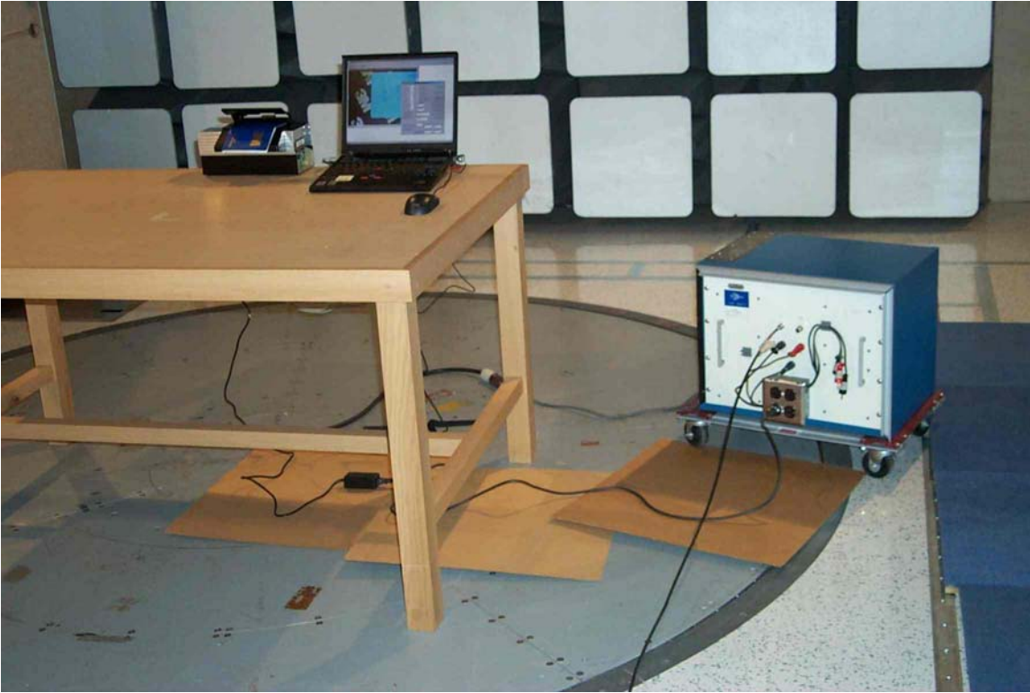
PV33 Conducted Emissions
