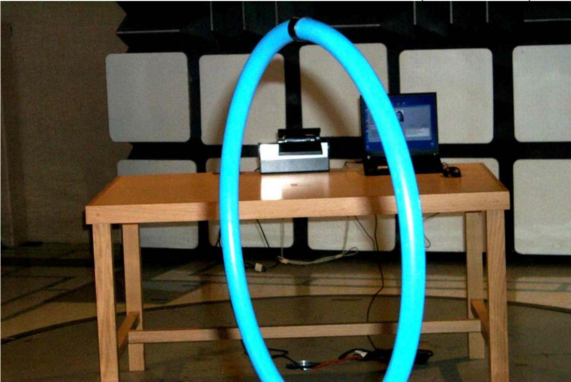
PV33 RFID Radiated Emissions and Emissions Bandwidth (9kHz – 30MHz)
