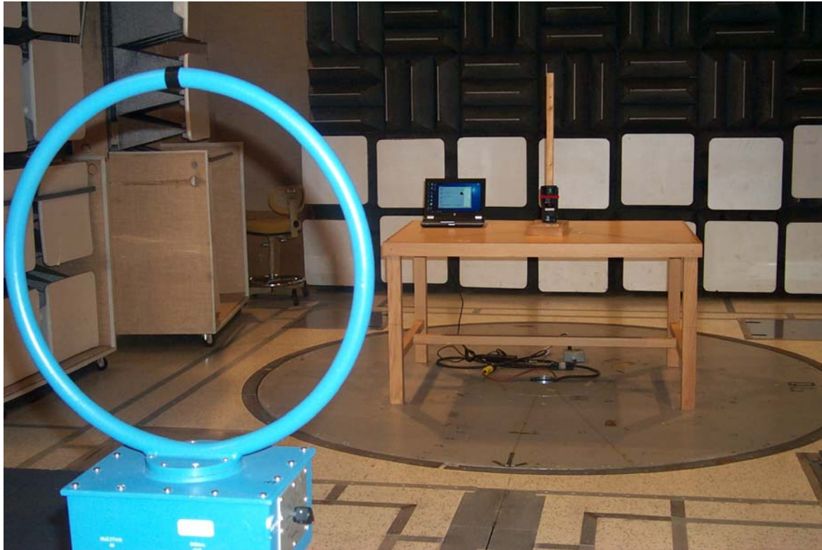
Carrier Frequency / Emissions Bandwidth / Spurious Emissions 9KHz to 30 MHz
