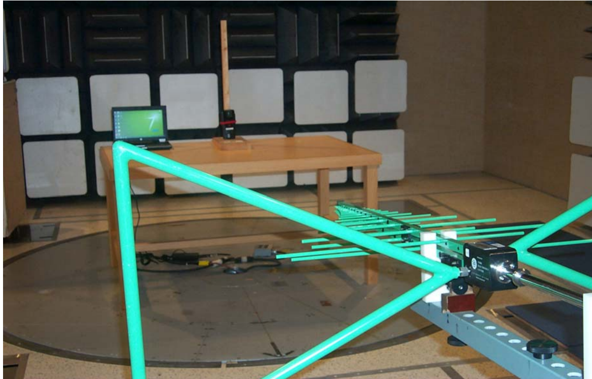
Radiated Emissions 30 to 1000 MHz
