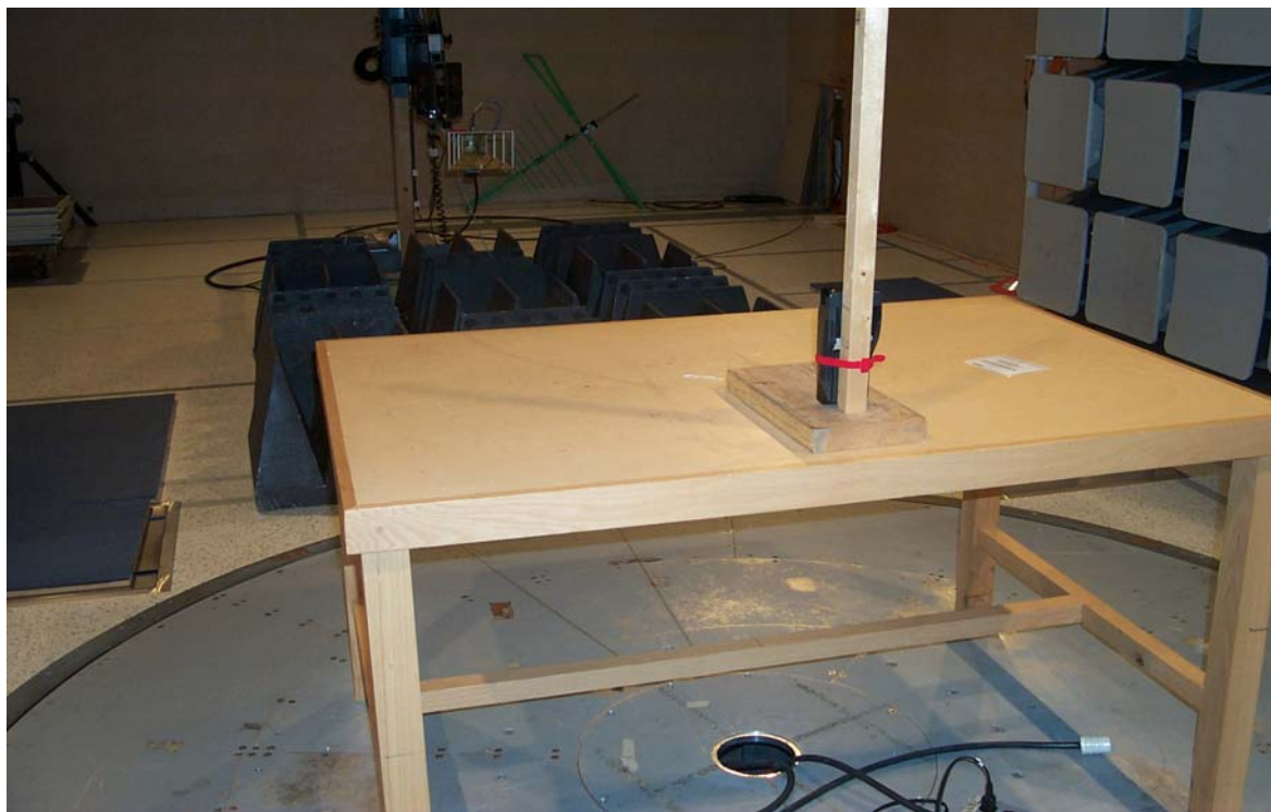
Radiated Emissions 1 to 18 GHz
