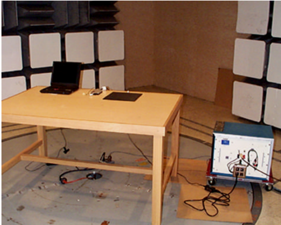
Conducted Emissions
