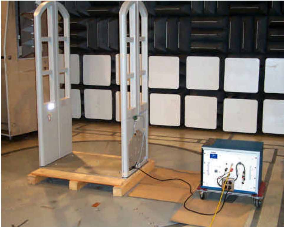
Conducted Emissions
