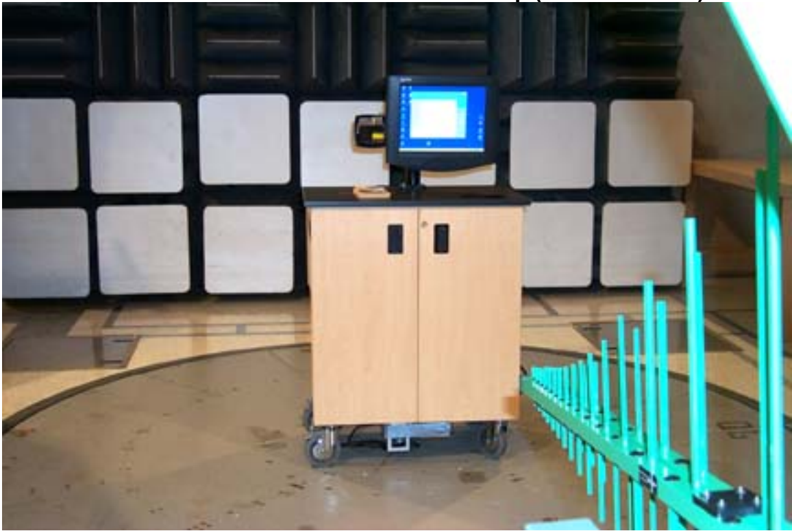
Model 812 Radiated Emissions Test Setup (80MHz – 1 GHz)
