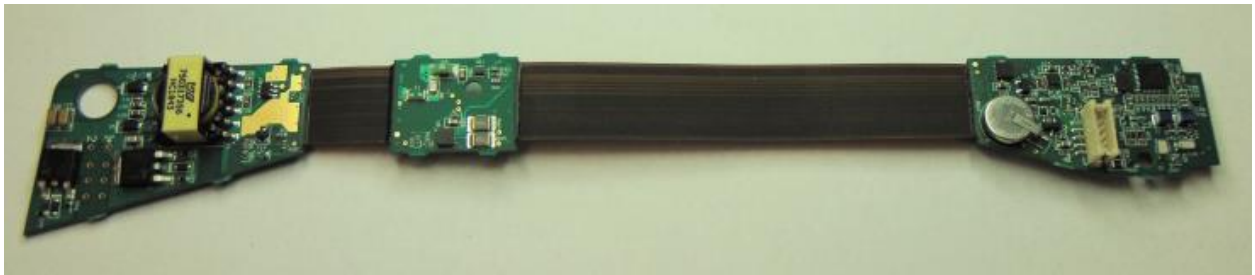
Chin-board Front
