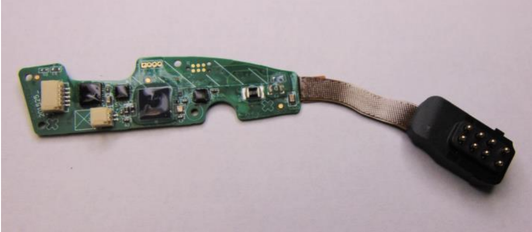
BCH Front
