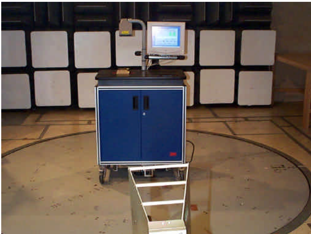
Radiated Emissions (1 to 5 GHz)
